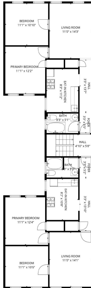
2nd Floor
