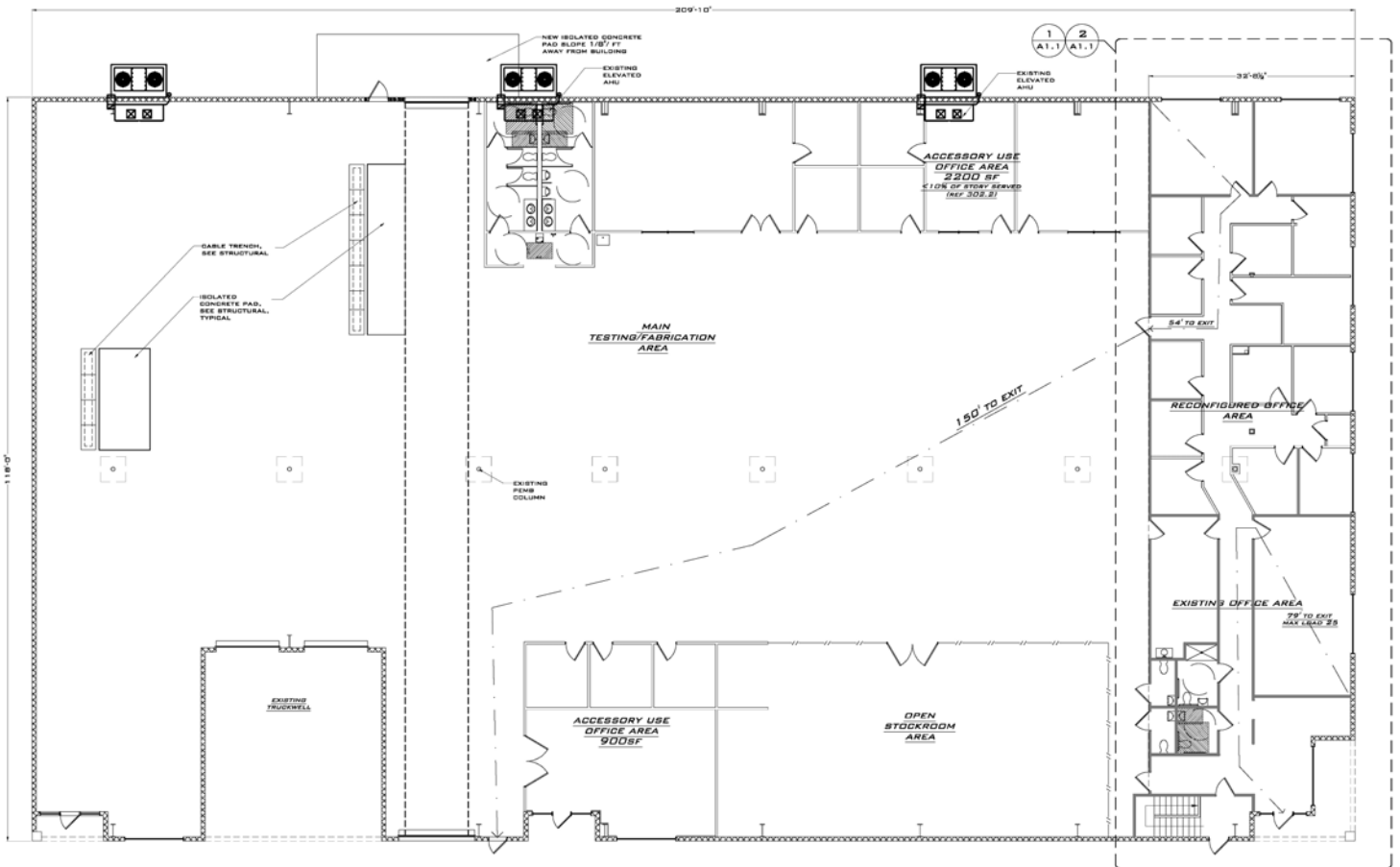
1 A1.1 PROPOSED FLOOR PLAN SCALE: 1/8" = 1'-0"
