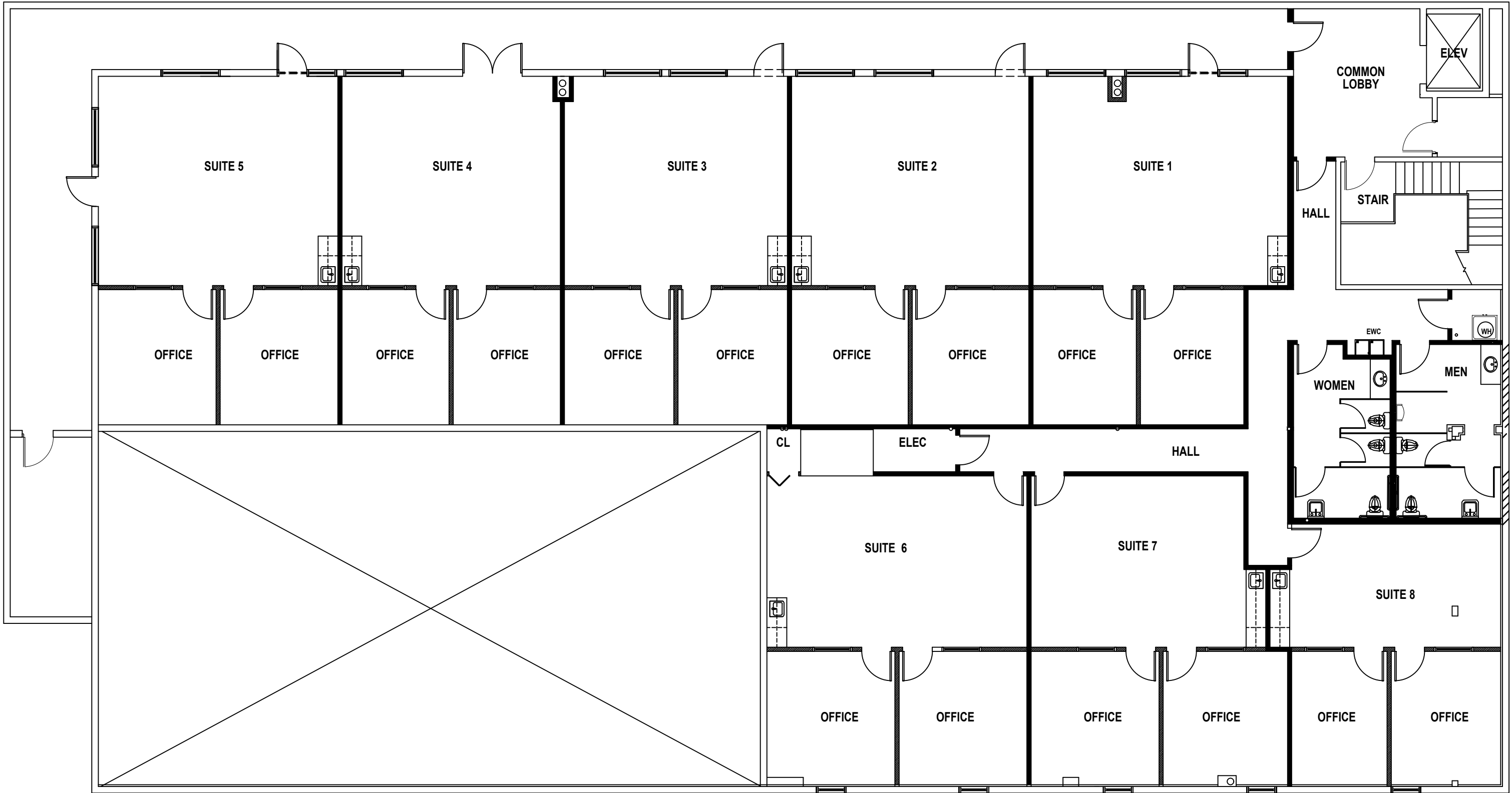
COVE BUILDING SECOND FLOOR PLAN
