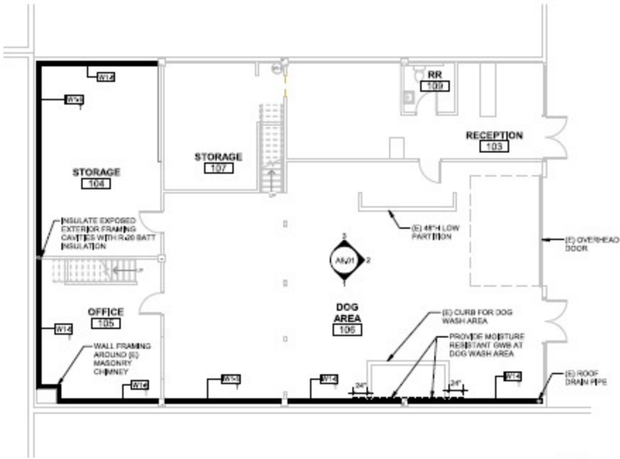
1 FIRST FLOOR PLAN 1/8" = 1'-0"
