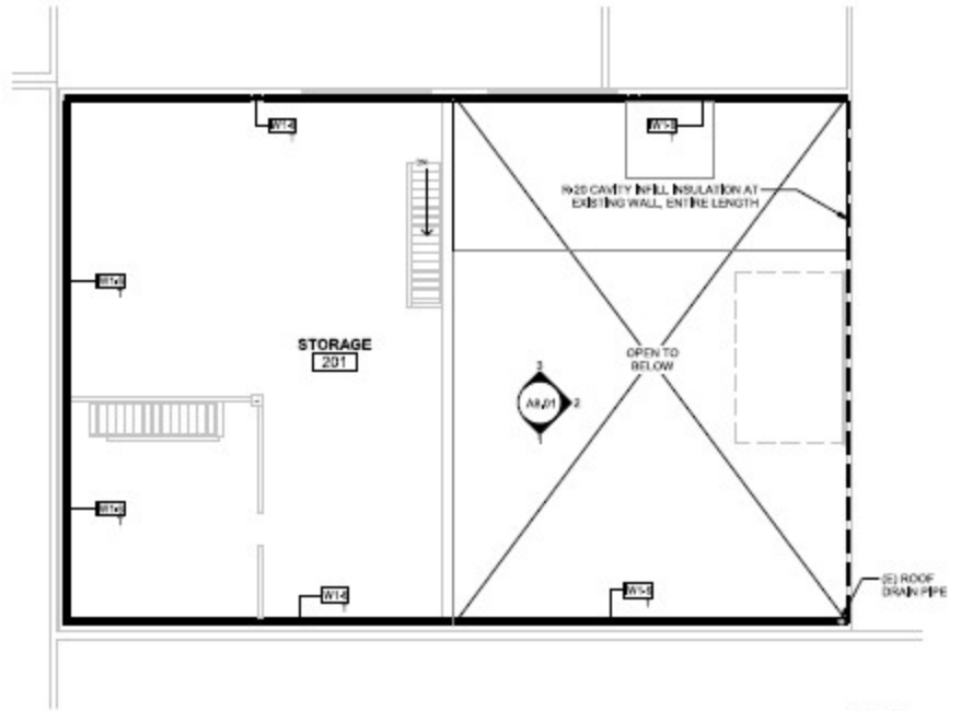
2 SECOND FLOOR PLAN 1/8" = 1'-0"
