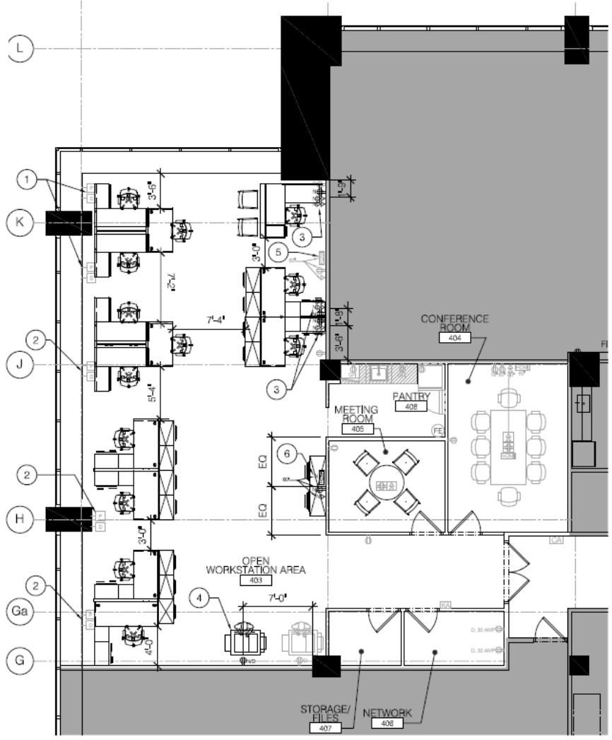
1 4TH FLOOR- FURNITURE & POWER PLAN 1/8" = 1'-0"
