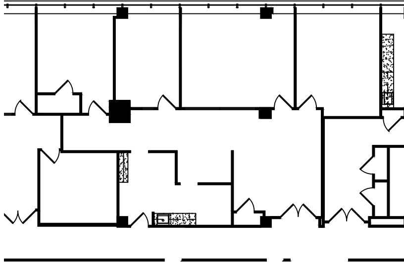
1 RECORD CONDITIONS SCALE: 1/16" = 1'0"
