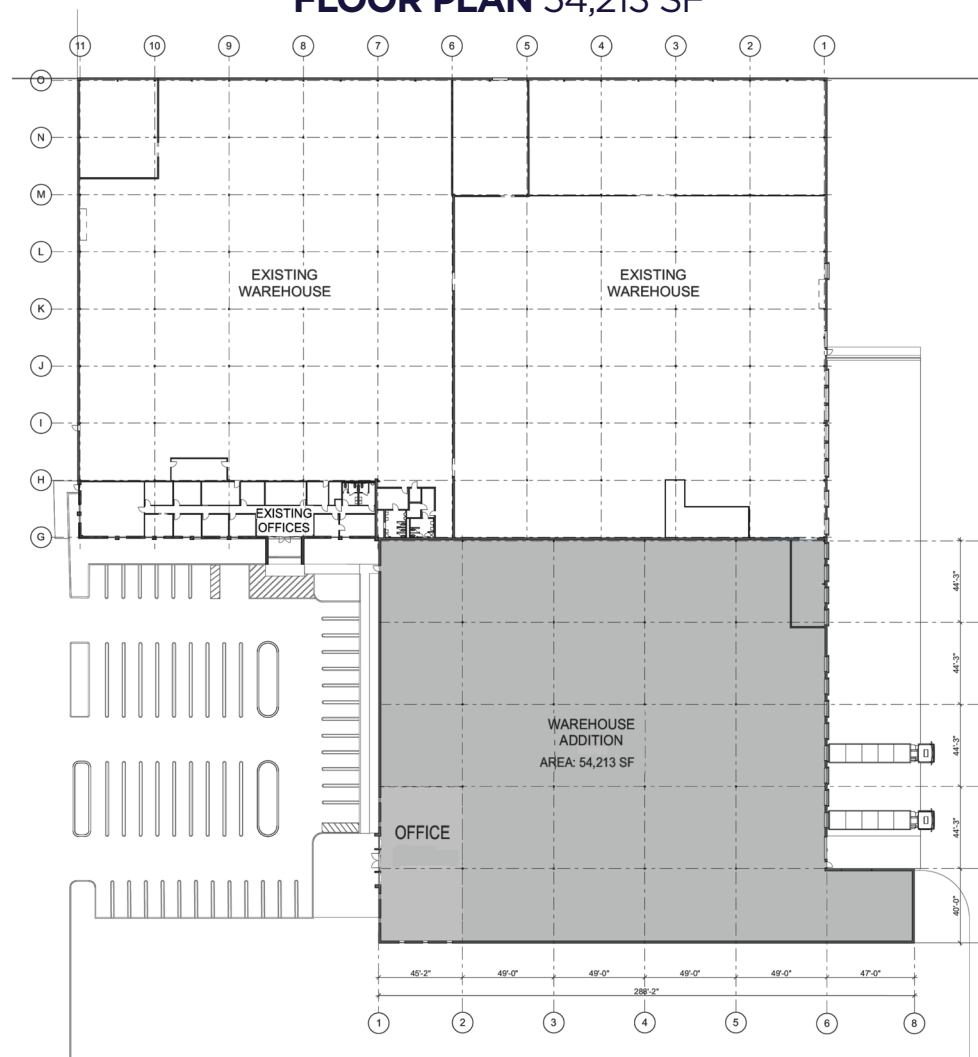
FLOOR PLAN 54,213 SF
