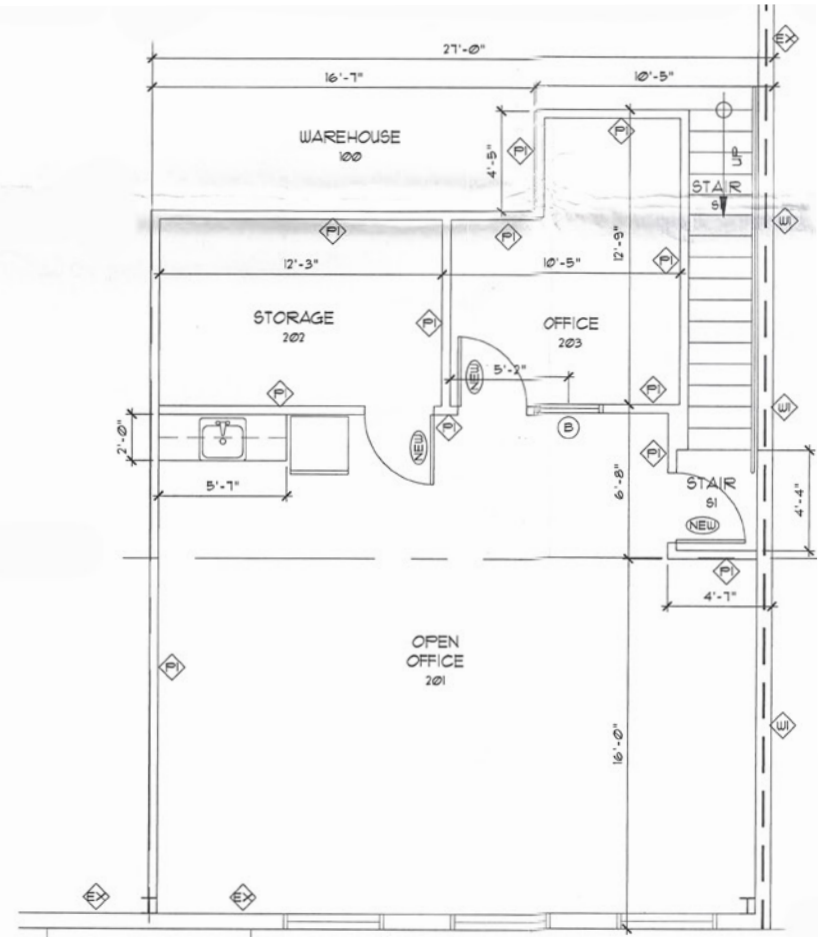
Mezzanine Floor Plan
