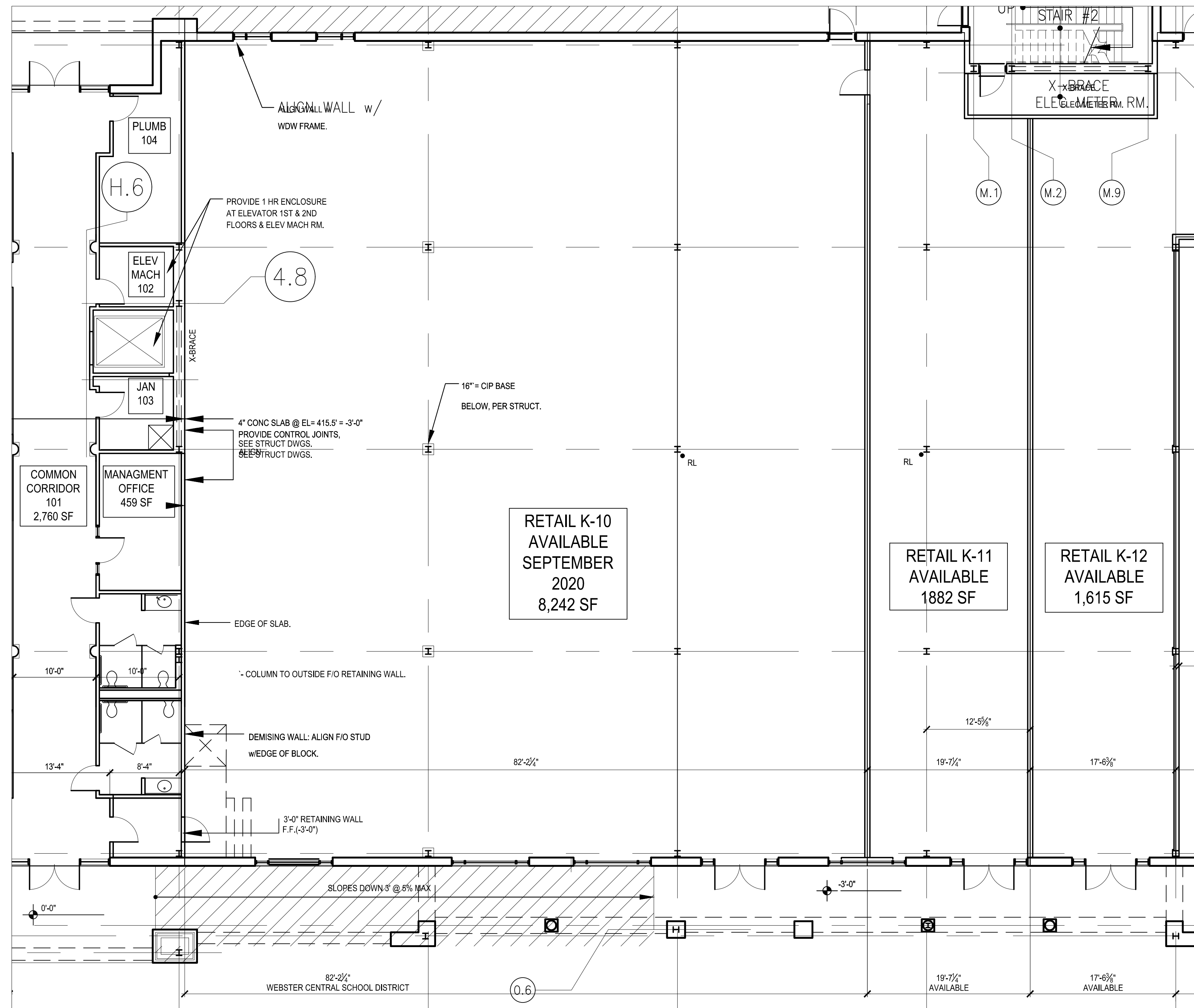
PARTIAL FLOOR PLAN \frac{1}{8}''=1'-0''
