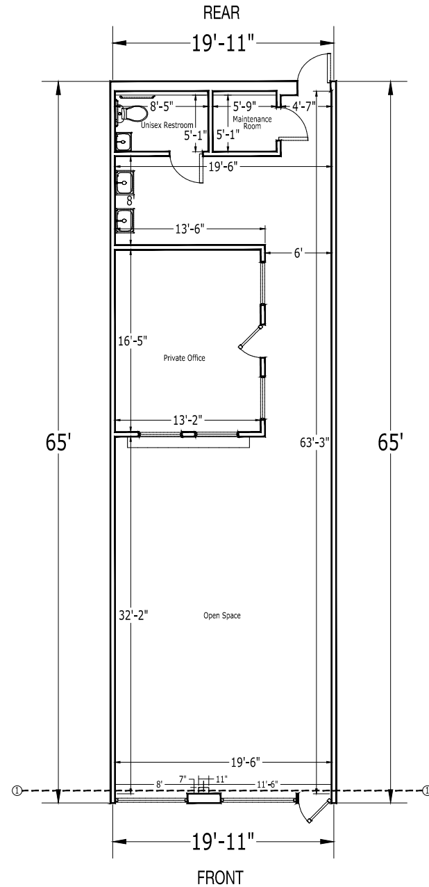
1 MAIN FLOOR
