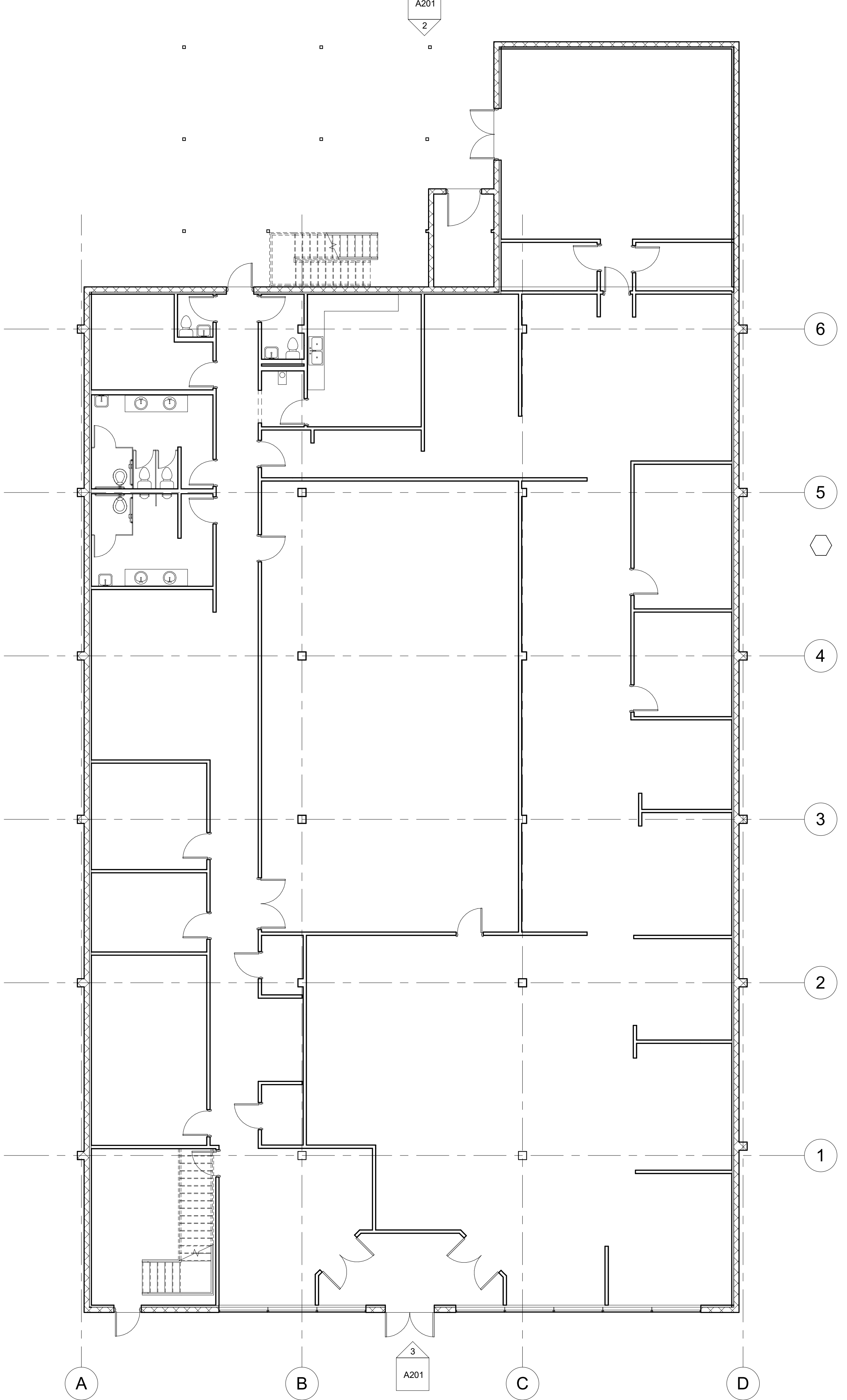
① OVERALL 1ST FLOOR PLAN 1/8" = 1'-0"
