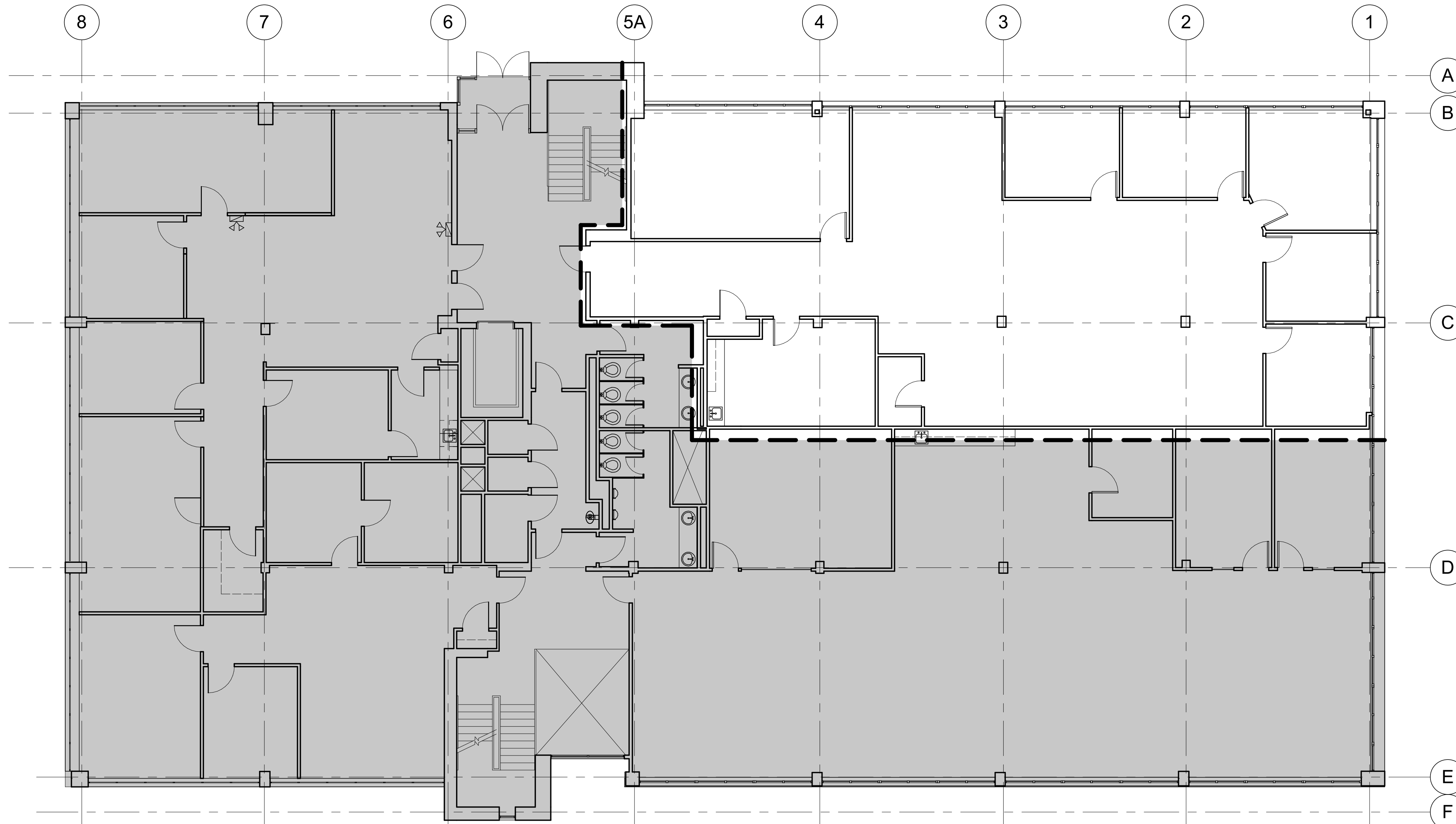
1 FIRST FLOOR EXISTING CONDITIONS PLAN SCALE: 1/8" = 1'-0"
