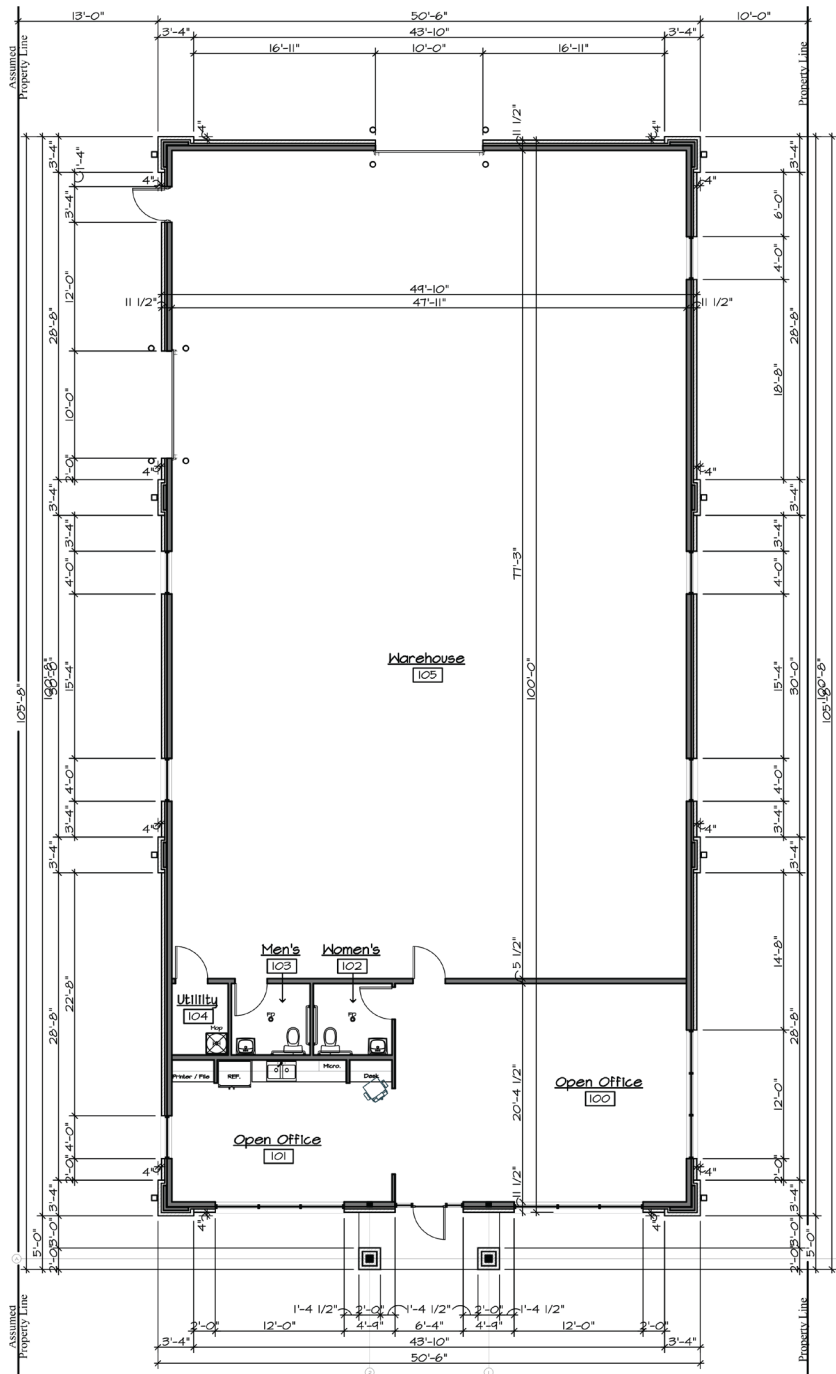
Floor Plan: Building '136'
