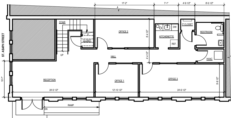
1 FIRST FLOOR PLAN Scale: 3/16" = 1'-0"
