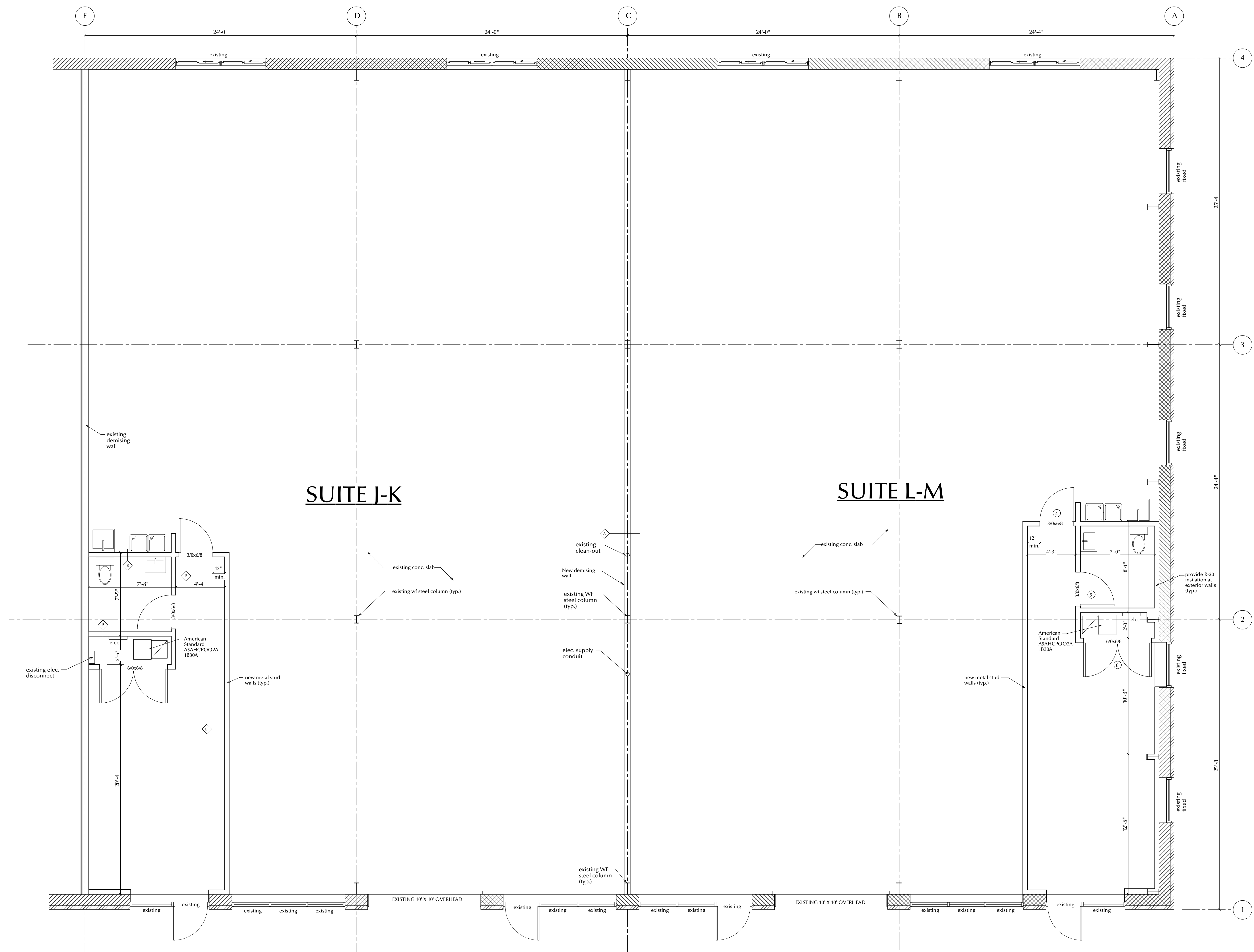
1 A-02 Proposed Floor Plan 1/4" = 1'-0"
