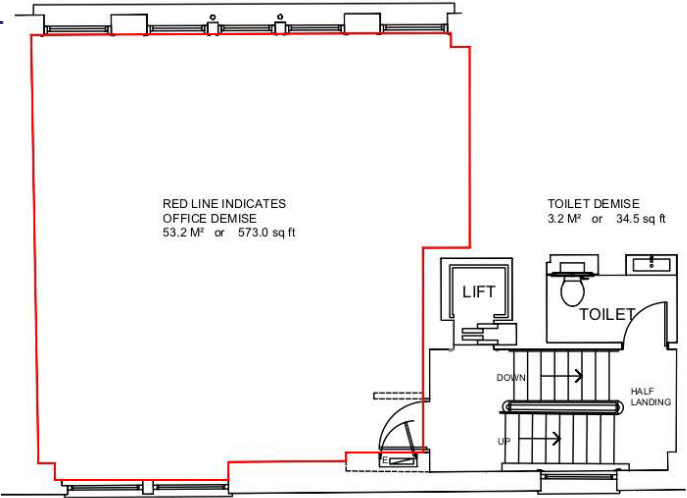
PROPOSED THIRD FLOOR PLAN
