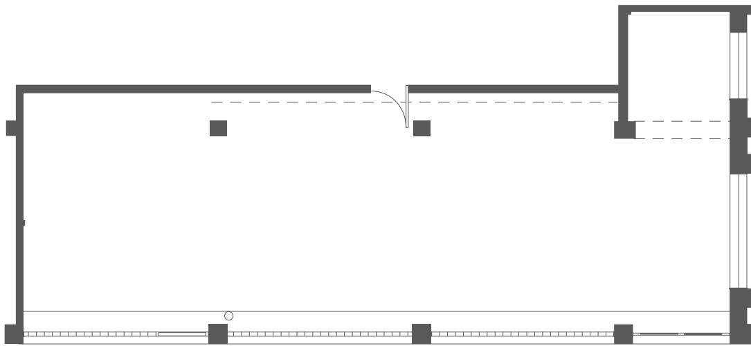
C-105 FLOOR PLAN
