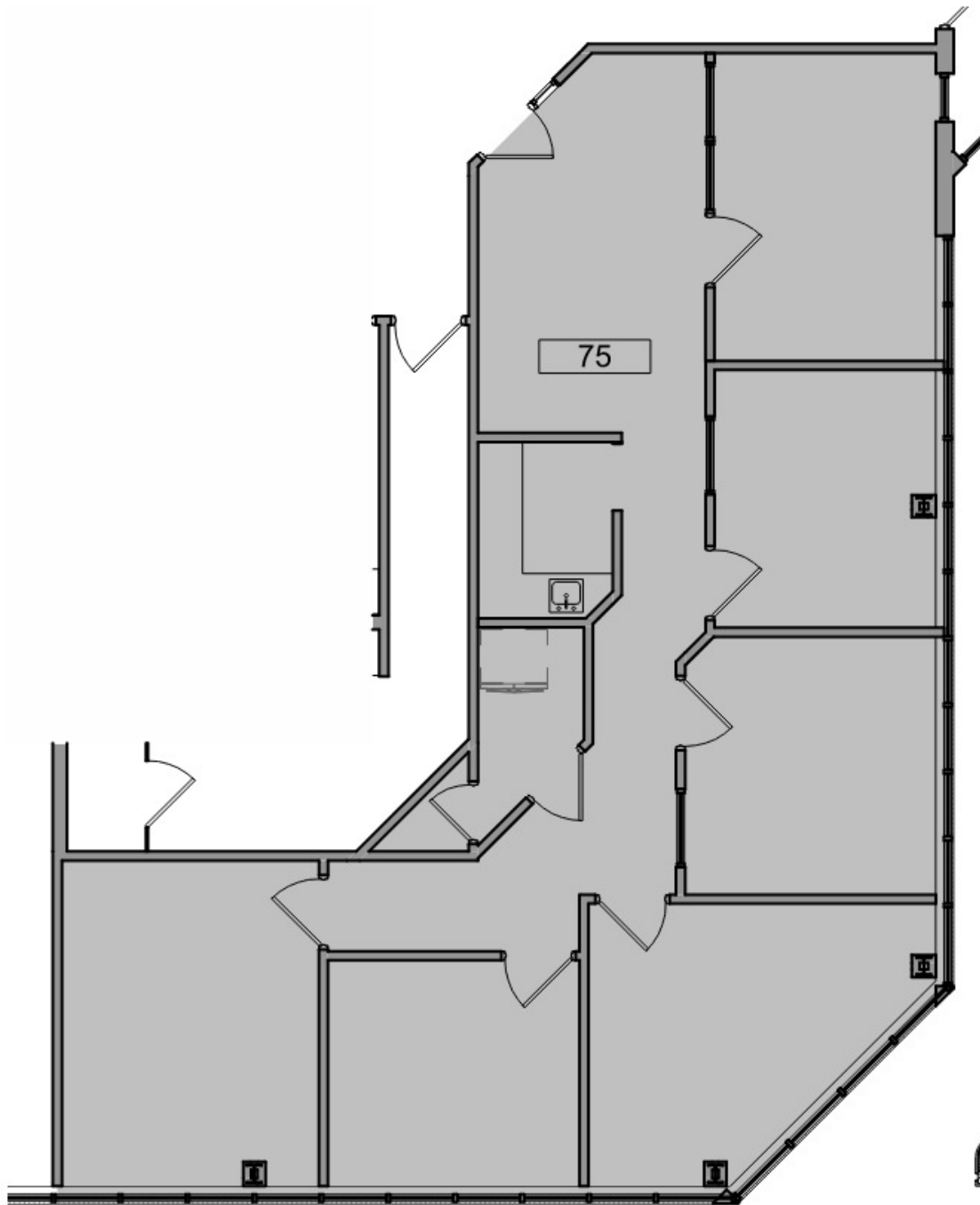
N 2 Suite 75 - Partial Terrace Level Existing Floor Plan 75 4' 8' 16' 1/8" = 1'-0"
