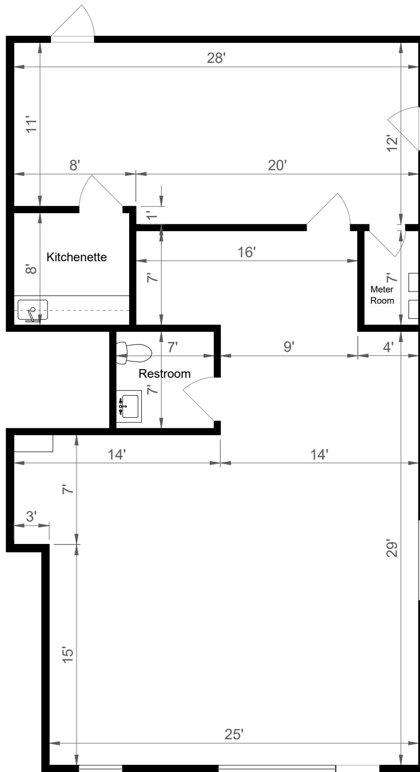
FLOOR PLAN
