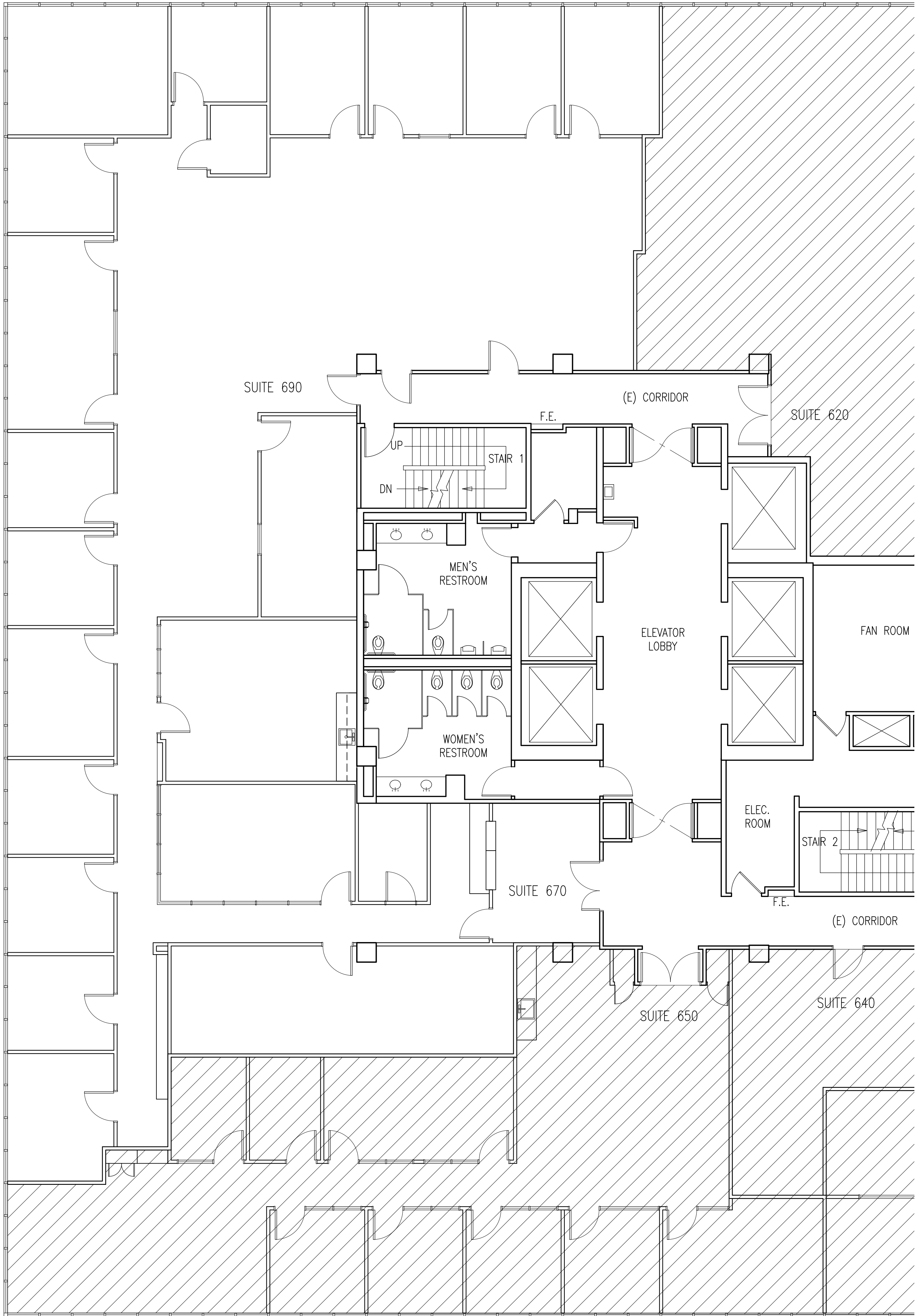
SUITE #670, #690 - AS-BUILT FLOOR PLAN 3055 Wilshire Blvd. NORTH Date: 08-07-25
