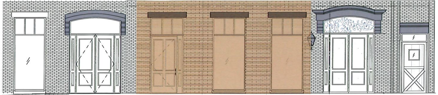
MOTT STREET ELEVATION
