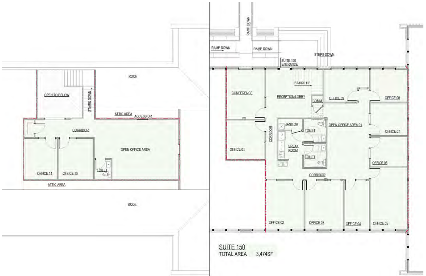
SECOND FLOOR
