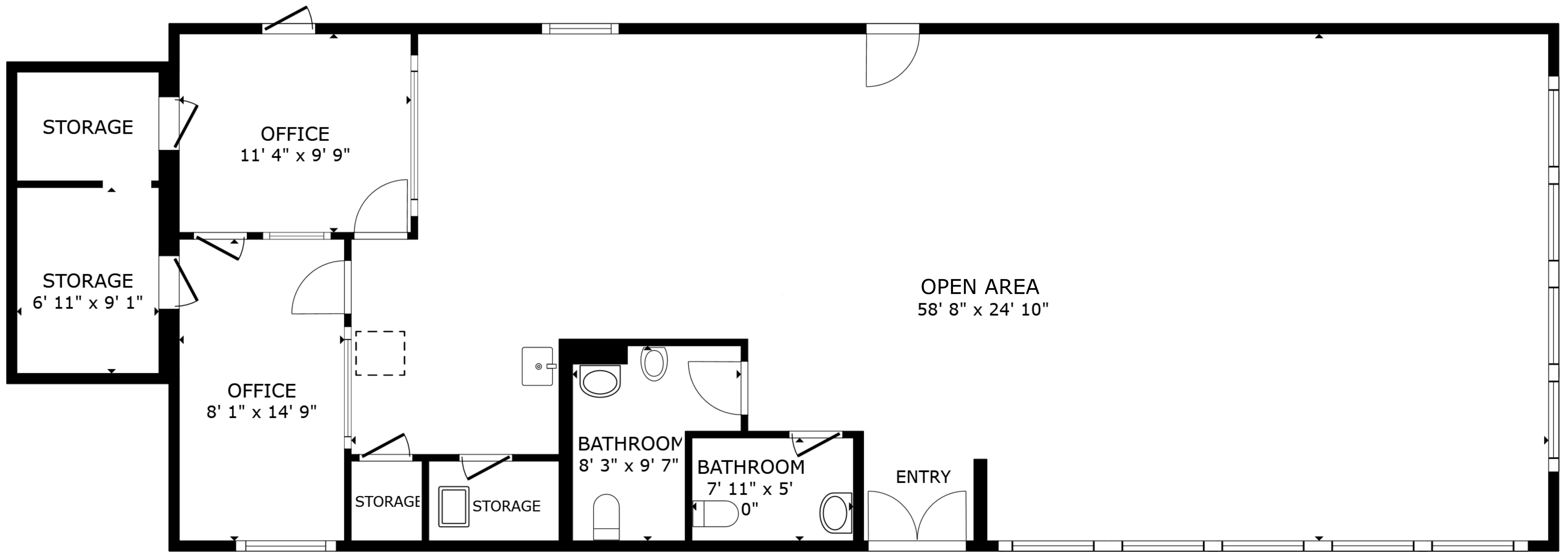
FLOOR PLAN
