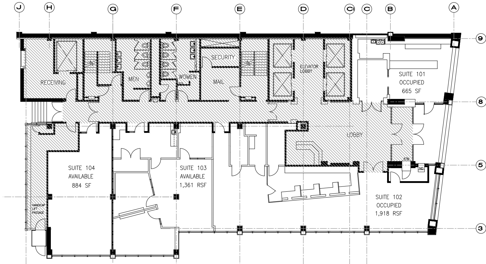
○ 1ST FLOOR PLAN SCALE: 1/16" = 1'-0" DATE: 4/16/24
