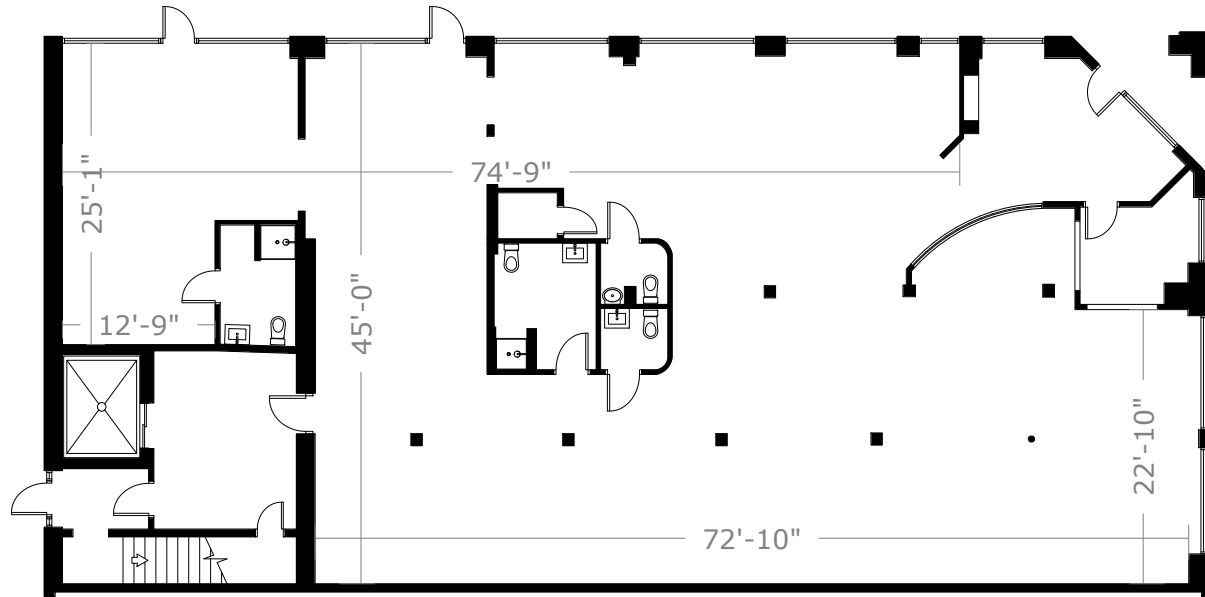
First Floor, 900 Central Ave | 1/16" = 1'-0"
