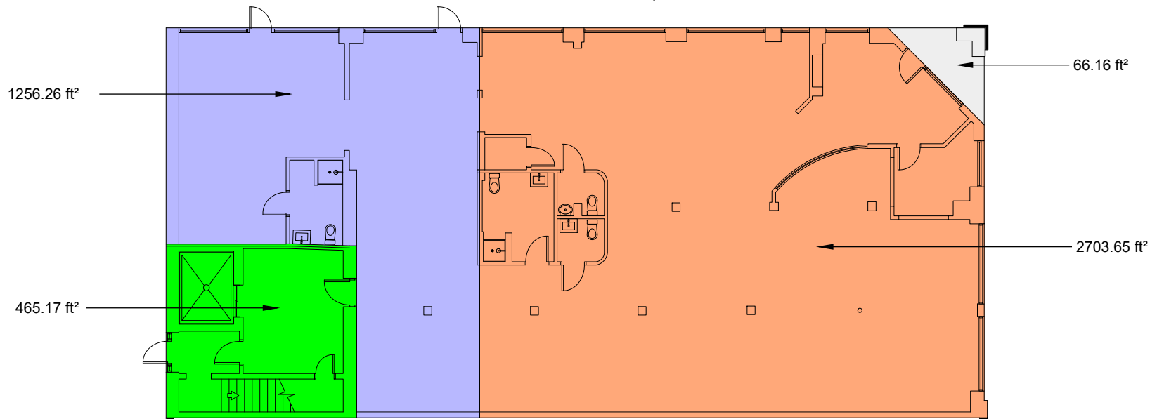
First Floor, 900 Central Ave | 1/16" = 1'-0"
