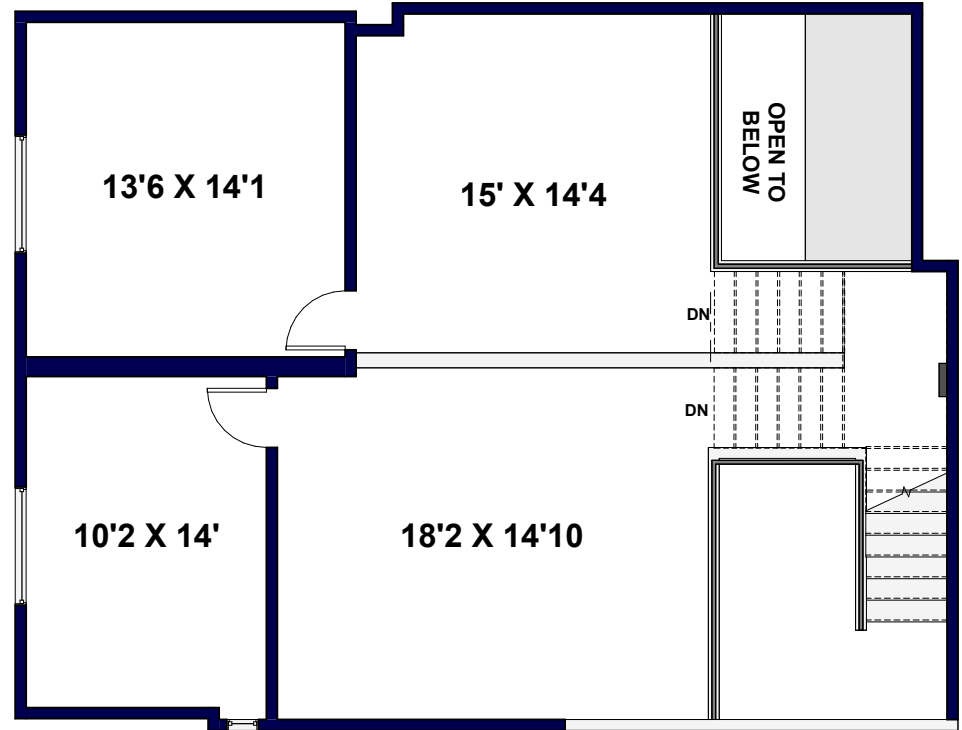
SECOND FLOOR
