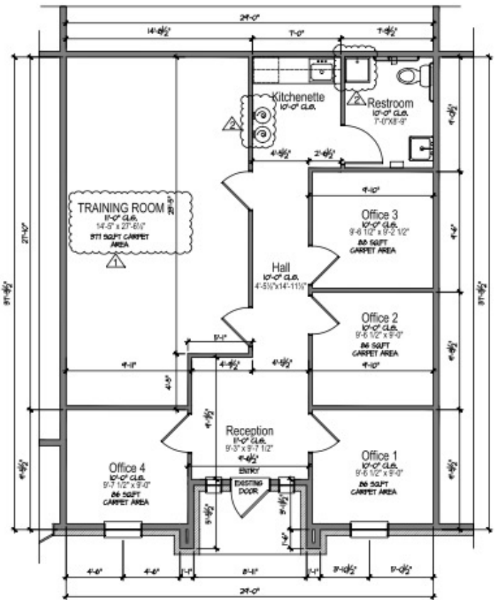
Dimensioned Floor Plan
