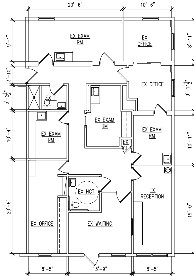
1 EXISTING FLOOR PLAN SUITE 6 SCALE: 1/8"=1'-0" 1,714 GSF
