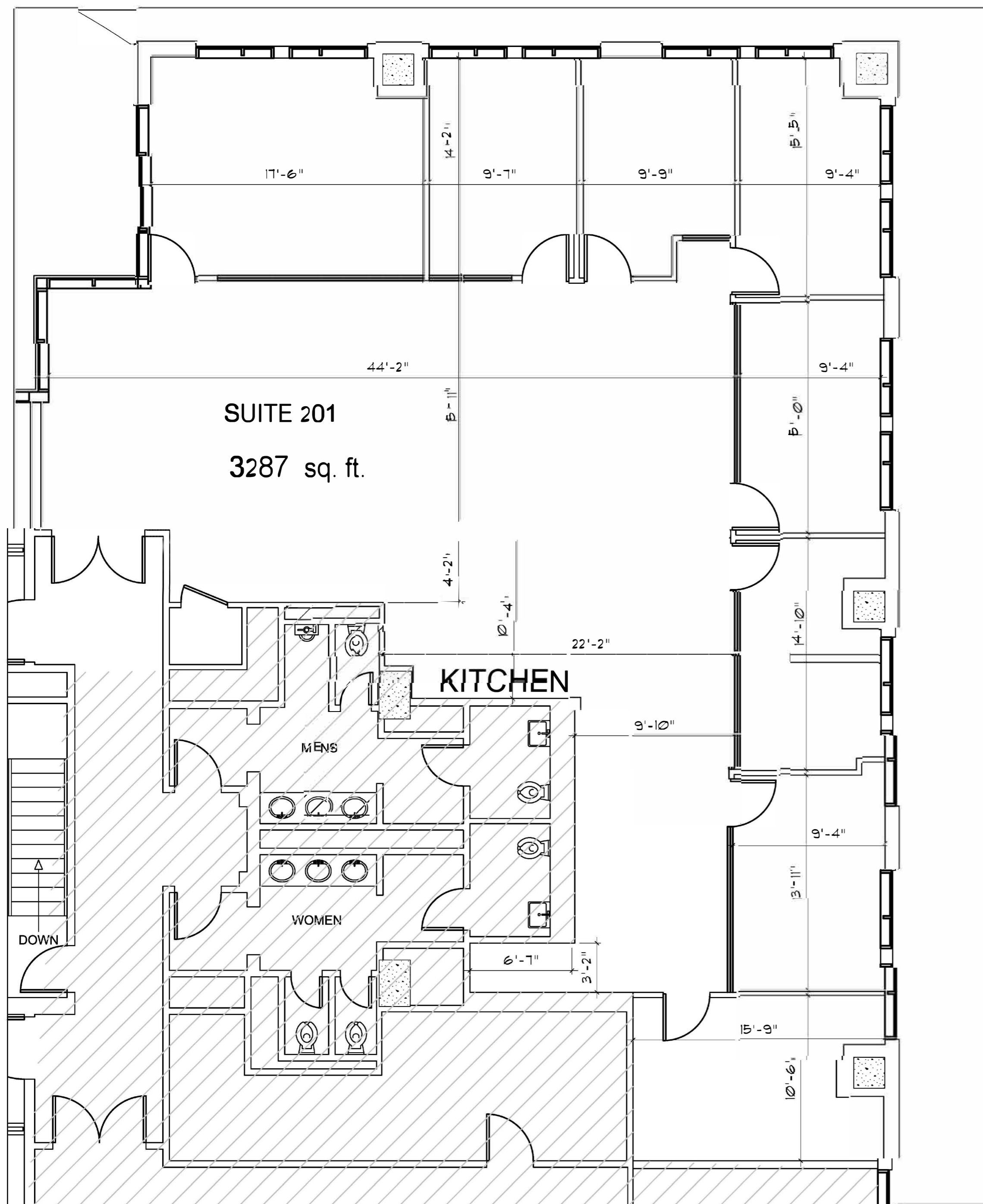
Floor Plan | Proposed
