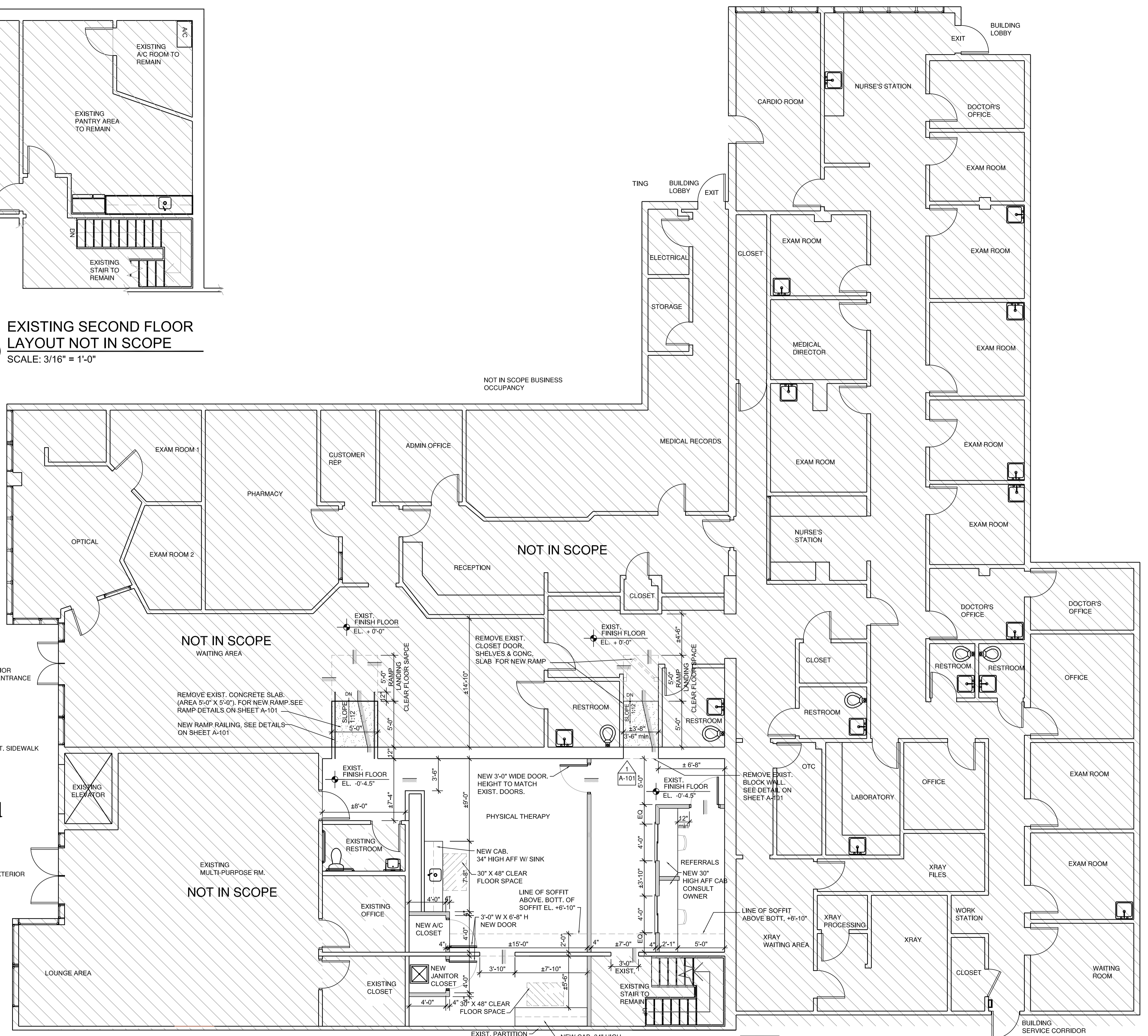
1 GROUND FLOOR LAYOUT SCALE: 3/16" = 1'-0"
