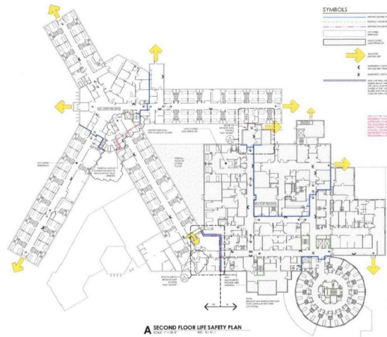
Second Floor Life Safety Plan
