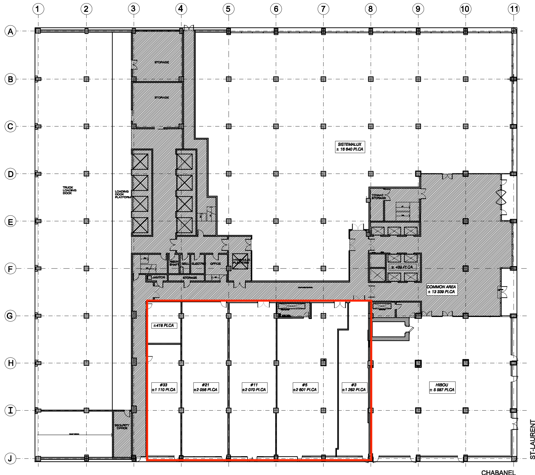
1 CHABANEL - GROUND FLOOR
