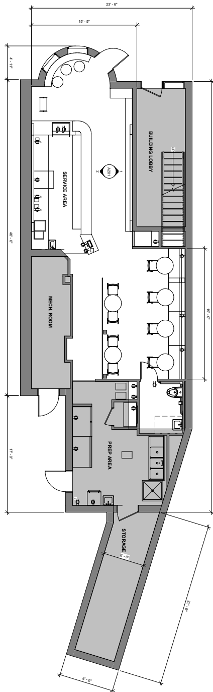
① LEVEL 1 PROPOSED FURNITURE PLAN 1/8" = 1'-0"
