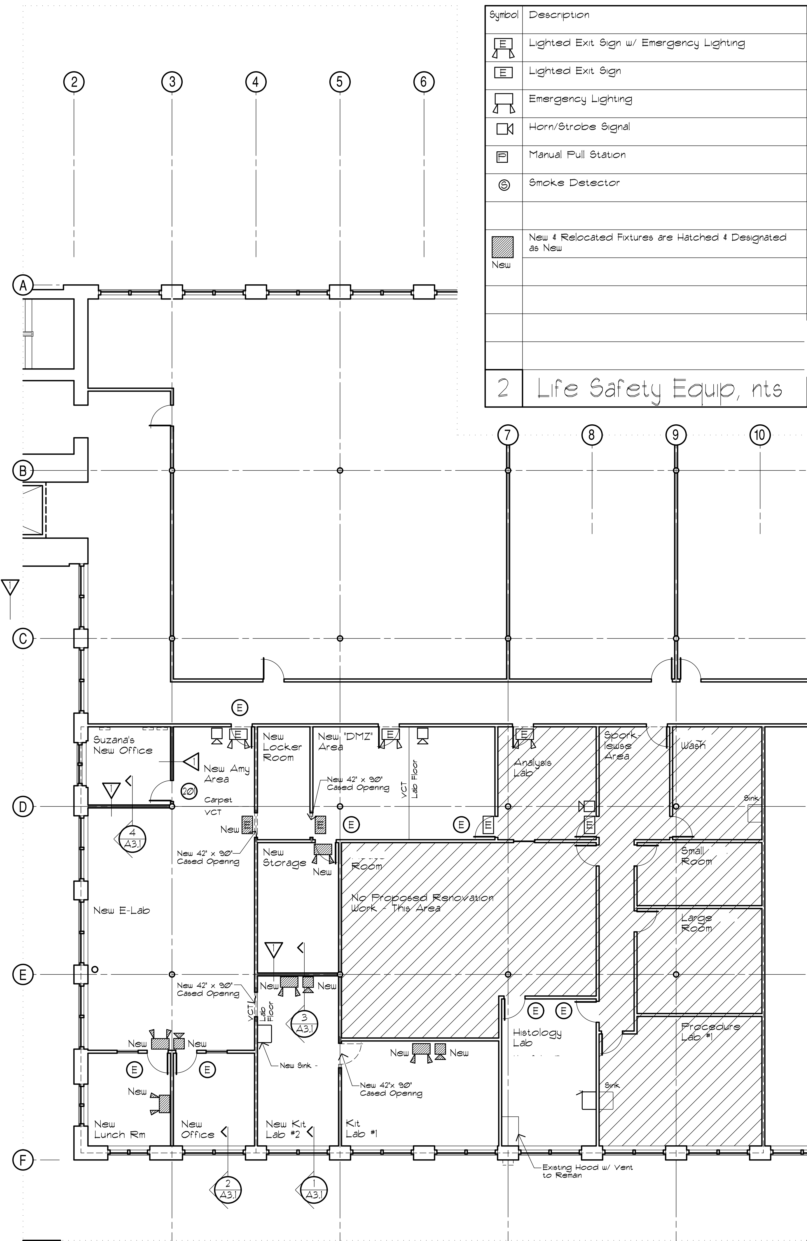
1 Partial Second Floor Plan - B2 (EC), 1/8" = 1'-0"
