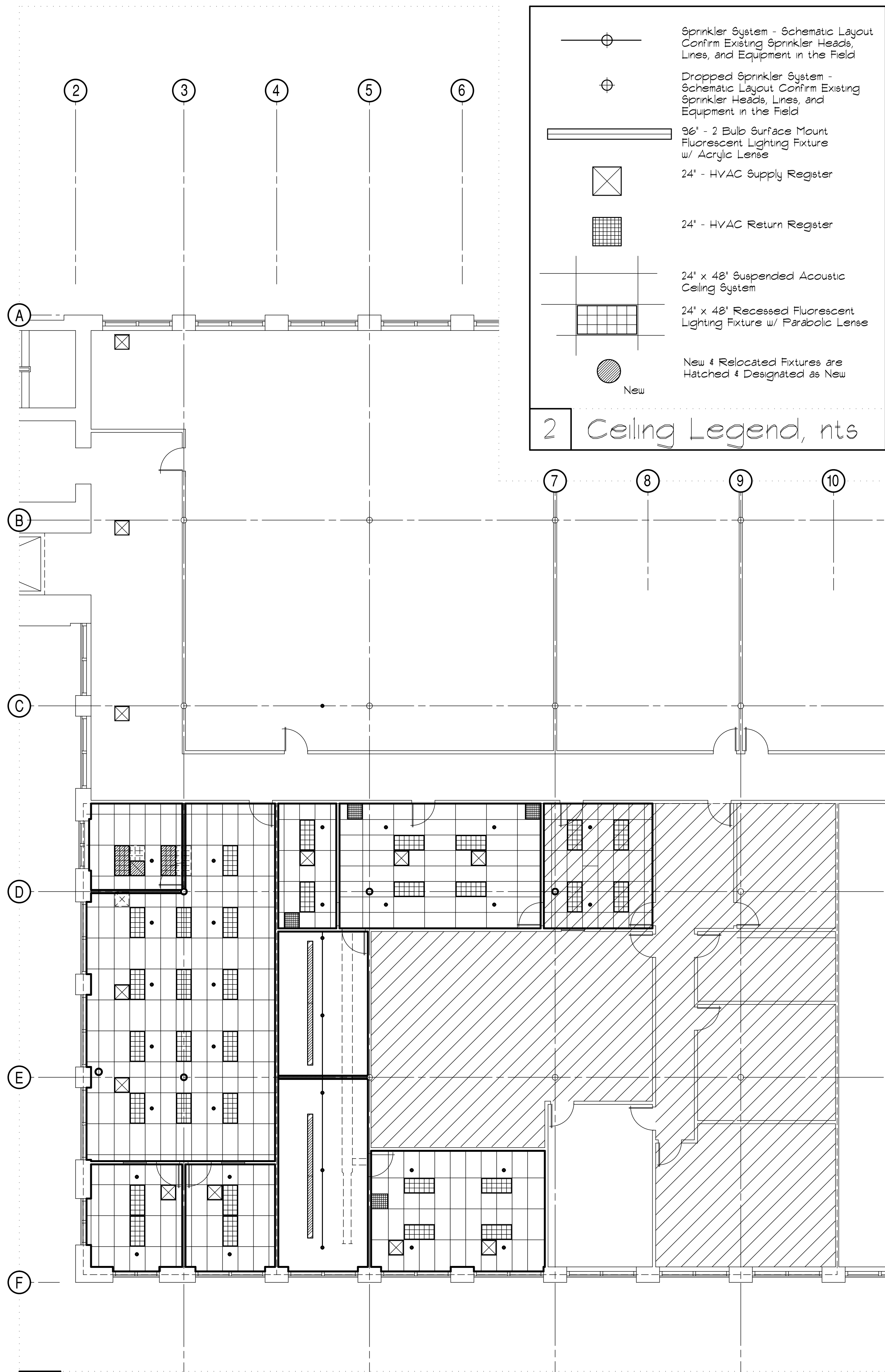
1 Partial Reflective Ceiling Plan - B2 (EC), 1/8" = 1'-0"
