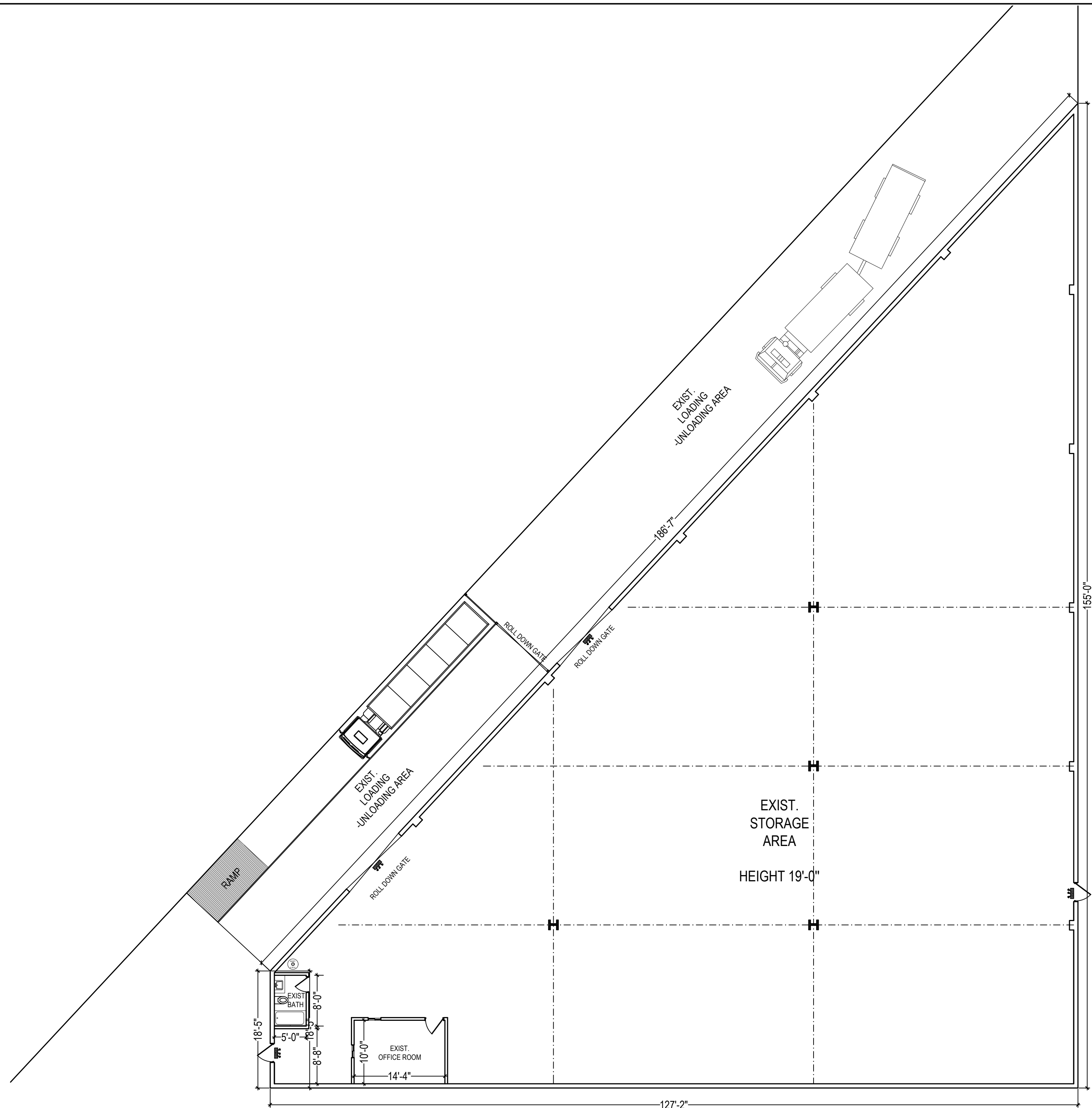
EXISTING 1ST FLOOR LAYOUT PLAN (AREA: 11,000 SF) SCALE: 3/32"=1'-0"
