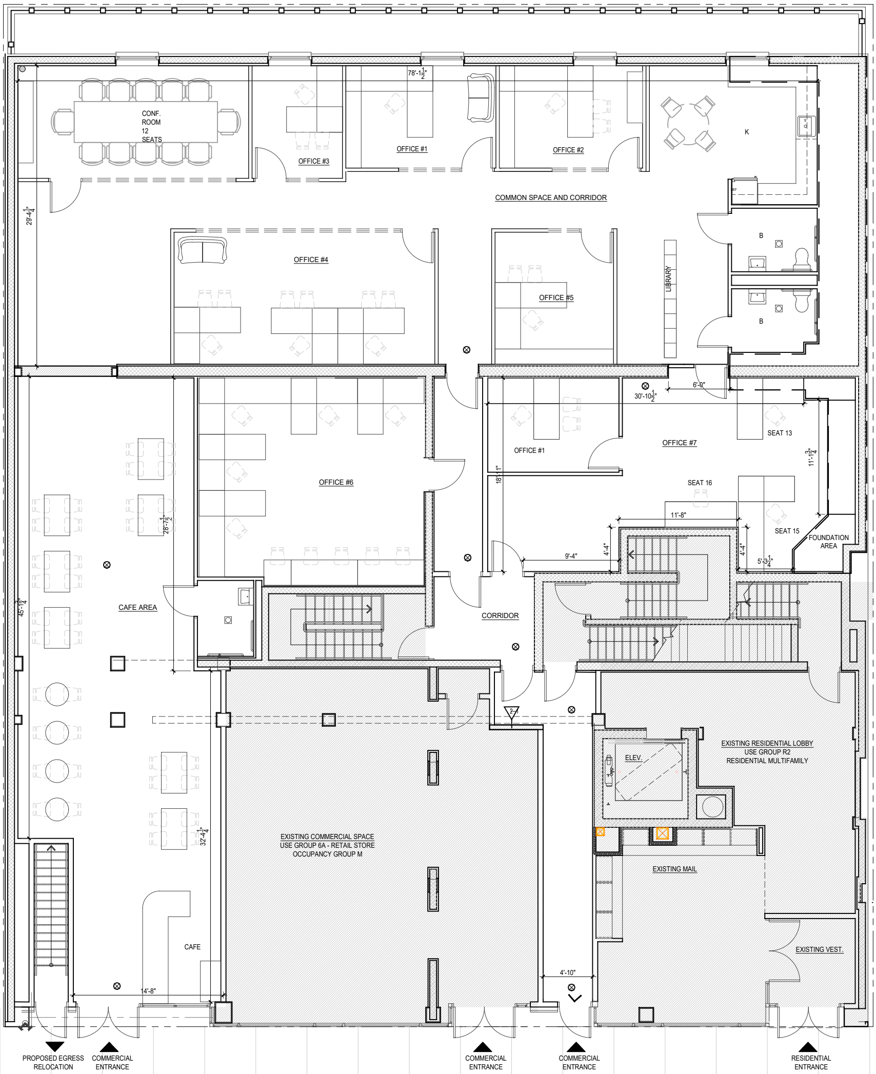
1ST FLOORPLAN - OPTION "C" NOT TO SCALE
