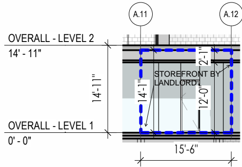
3 ELEVATION - RETAIL R05 LOD SCALE: 1/16" = 1'-0"
