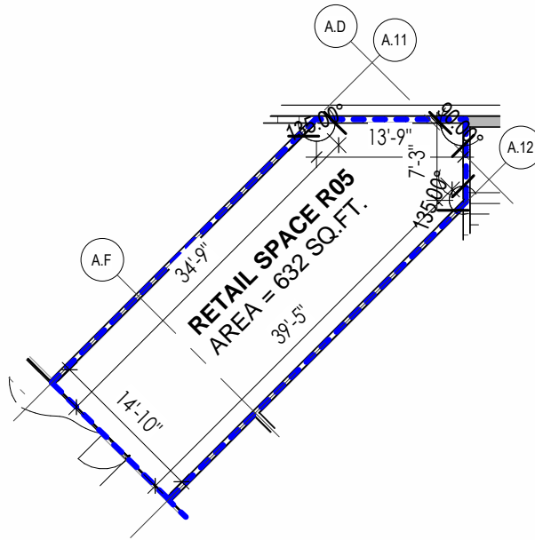
2 RETAIL SPACE - R05 SCALE: 1/16" = 1'-0"
