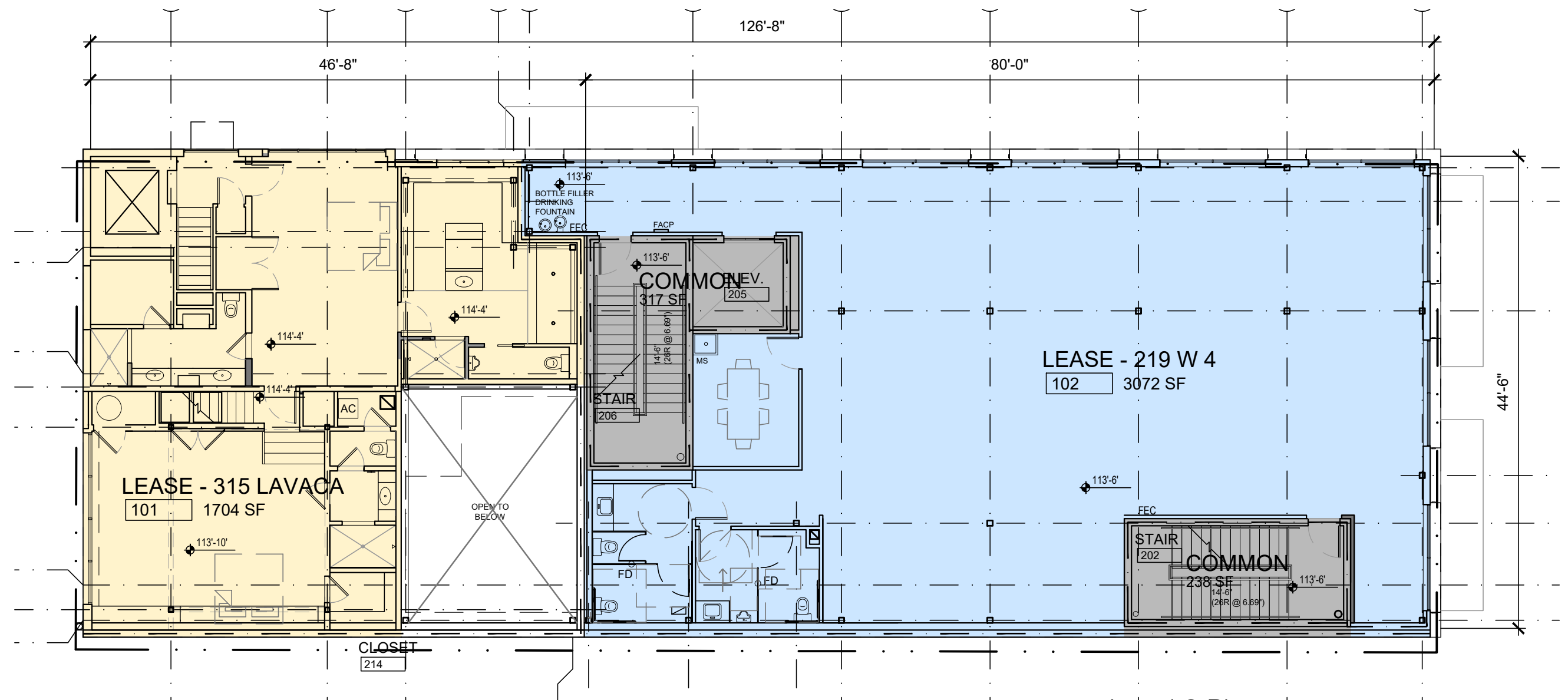
Level 2 Plan
