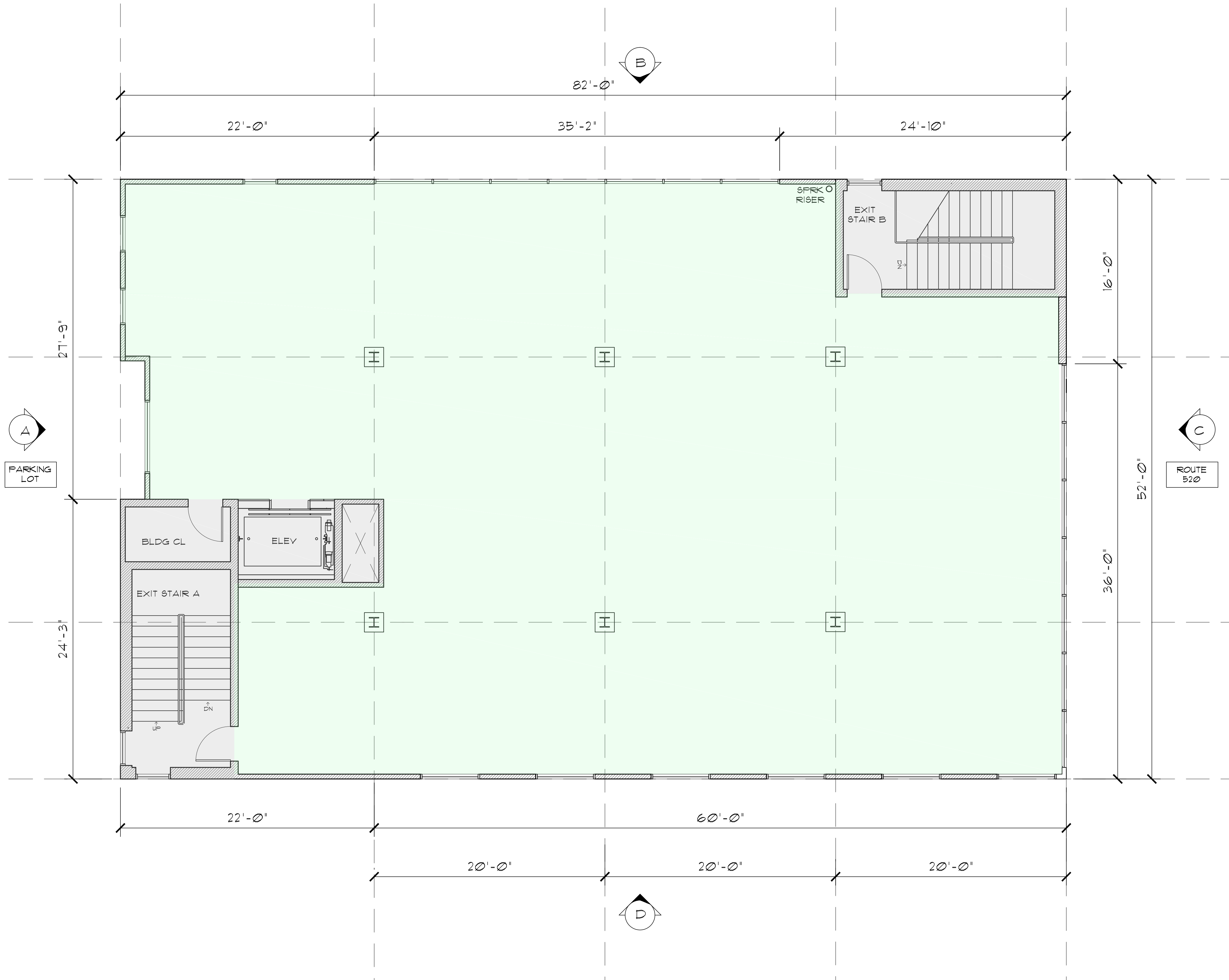
PROPOSED THIRD FLOOR PLAN
