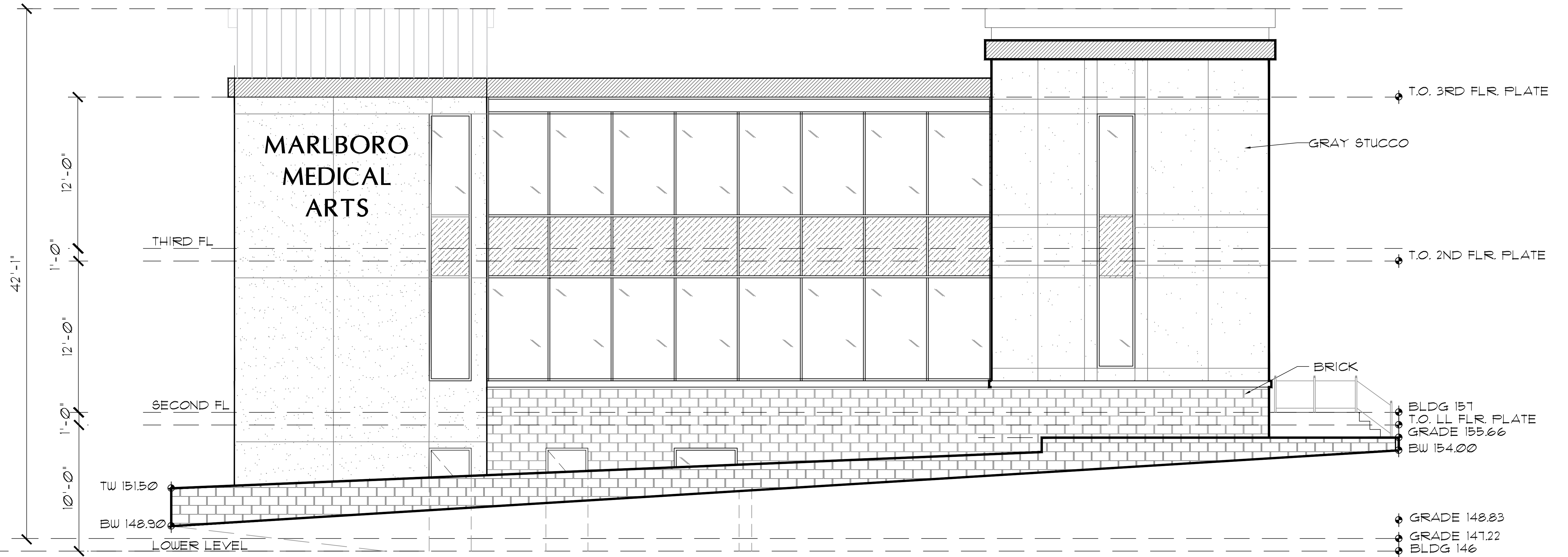
(B) WEST ELEVATION
