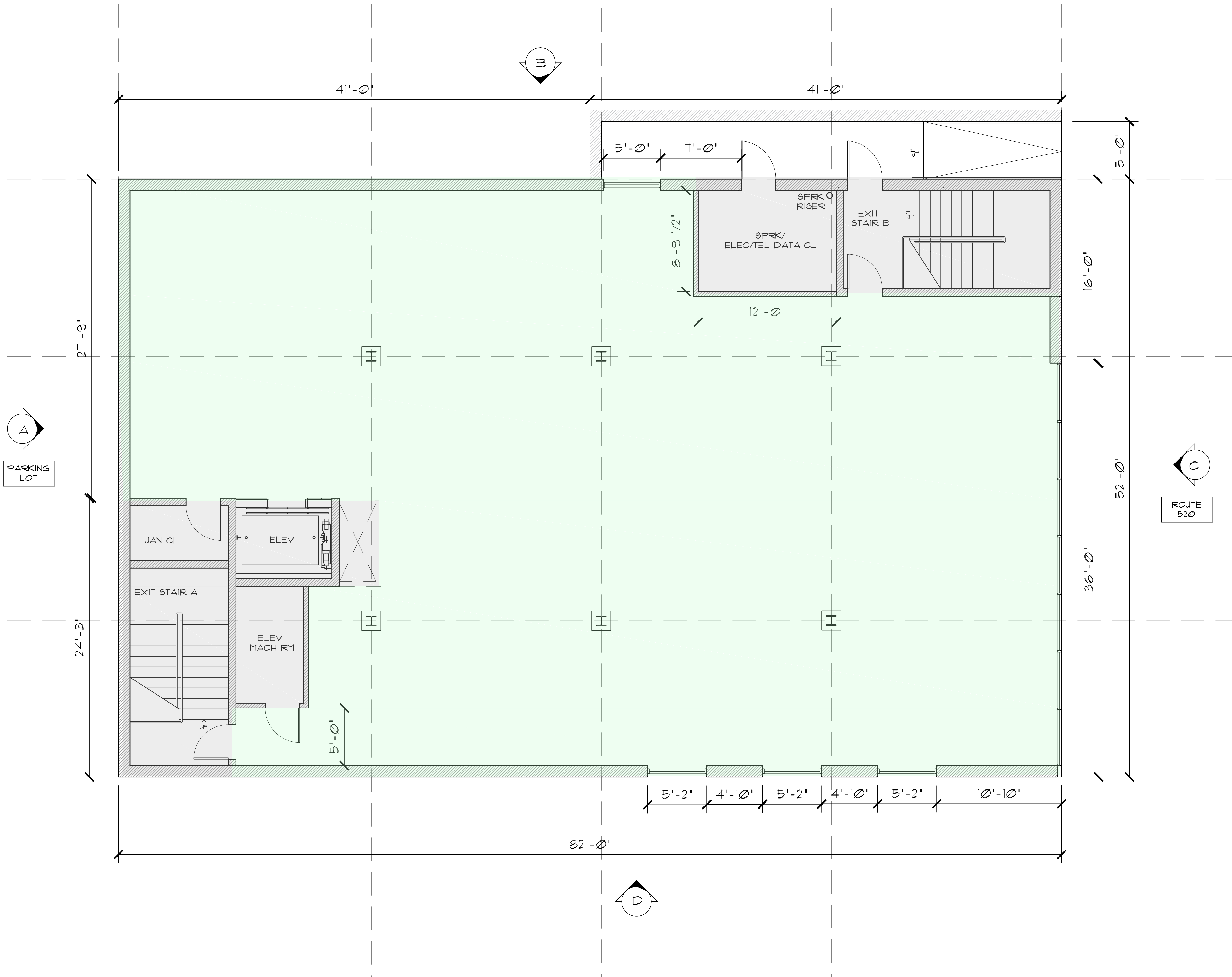
PROPOSED LOWER LEVEL PLAN
