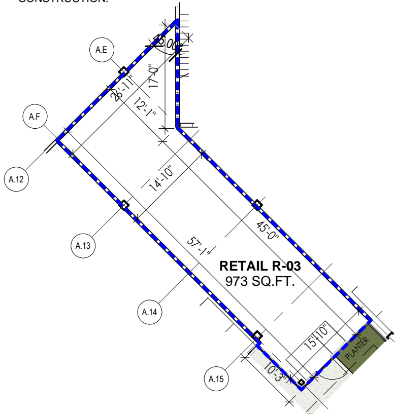
2 RETAIL SPACE R-03 LOD SCALE: 1/16" = 1'-0"
