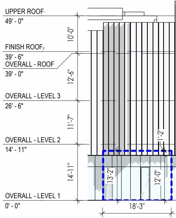
3 EAST ELEVATION- RETAIL R03 SCALE: 1/16" = 1'-0"
