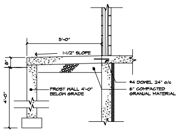
X SECTION at ENTRANCE SCALE: 3/4" = 1'-0"
