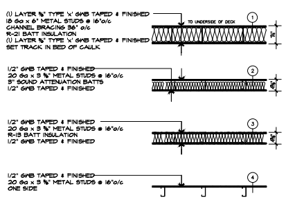
PARTITION SCHEDULE SCALE: 3/4" = 1'-0"
