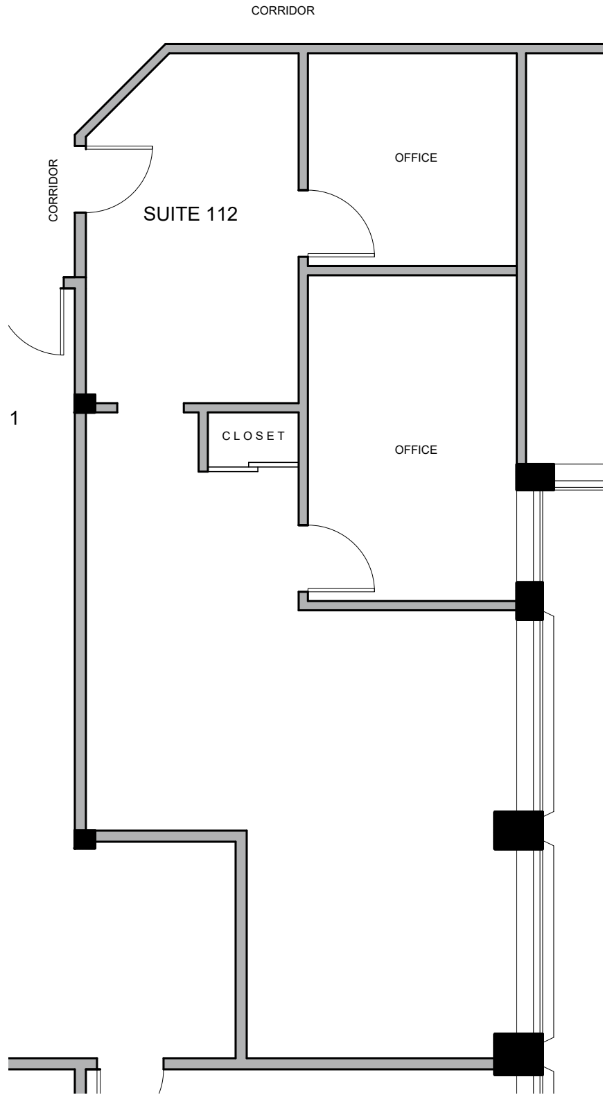
- 1st FLOOR PART PLAN (SUITE 112) - 1/4" = 1'-0" AREA: 954 R.SQ.FT
