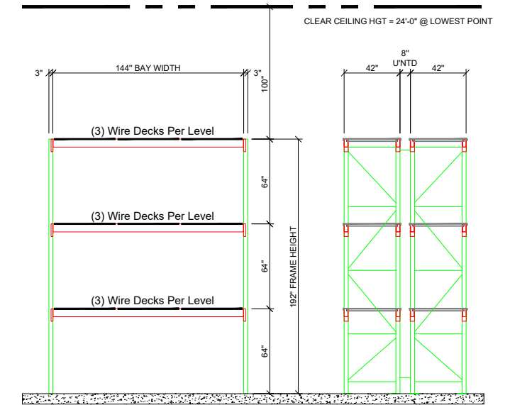
TYPICAL BEAM PROFILE (NTS)
