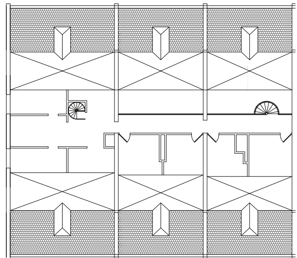
UPPER MEZZANINE
