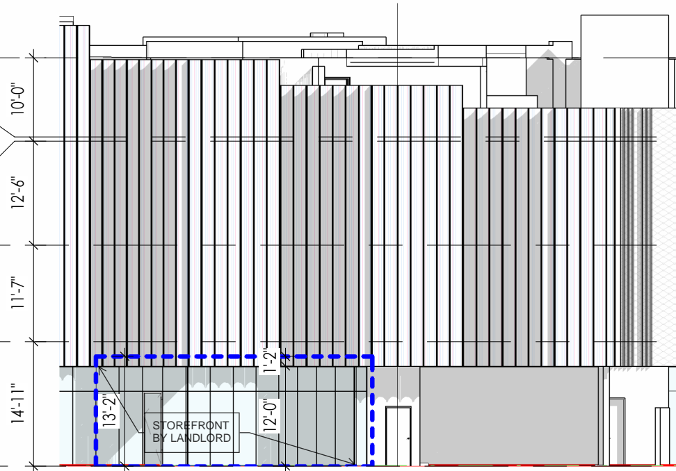
3 NORTH ELEVATION - RETAIL R01 SCALE: 1/16" = 1'-0"
