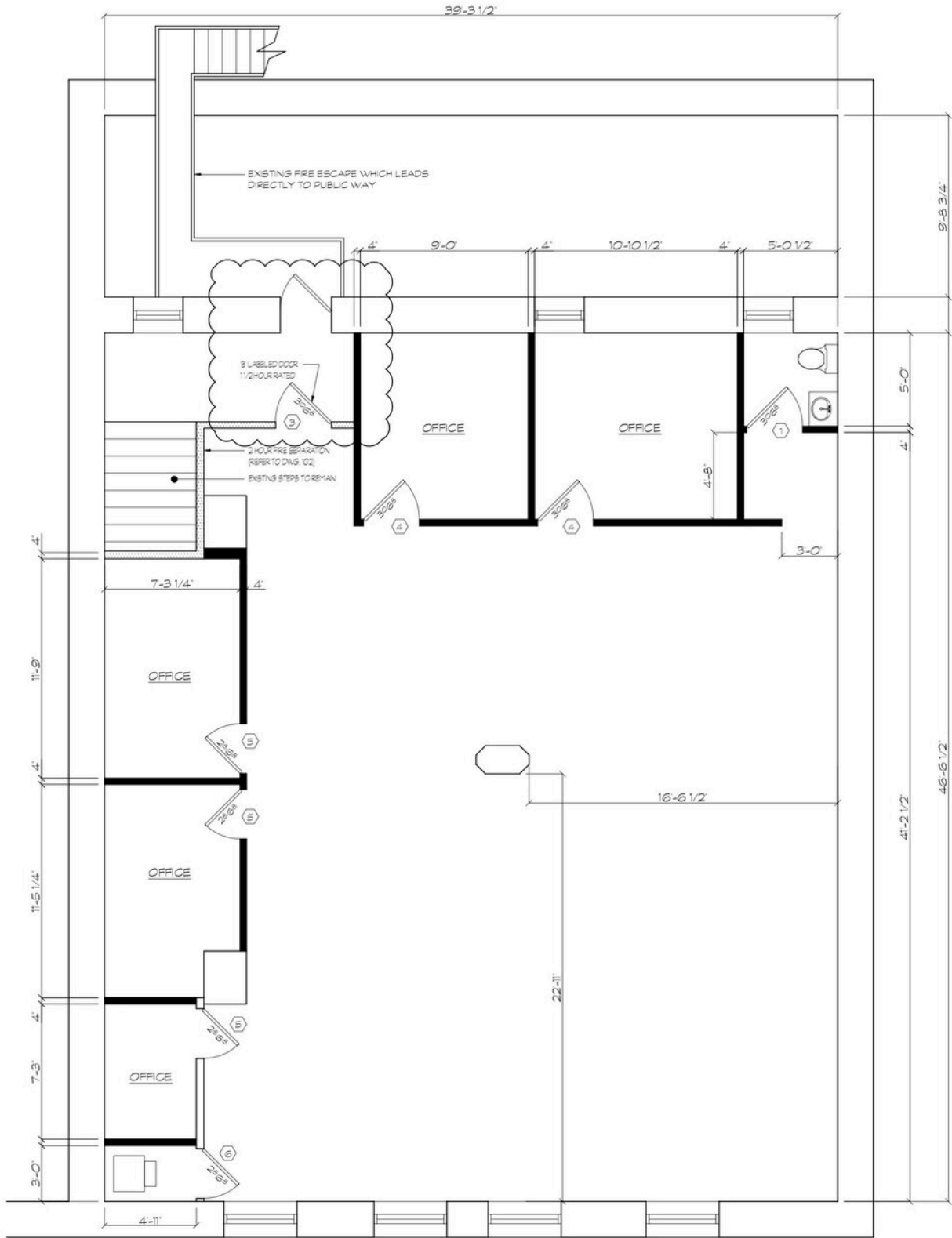
PROPOSED THIRD FLOOR PLAN SCALE 3/16" = 1'-0"
