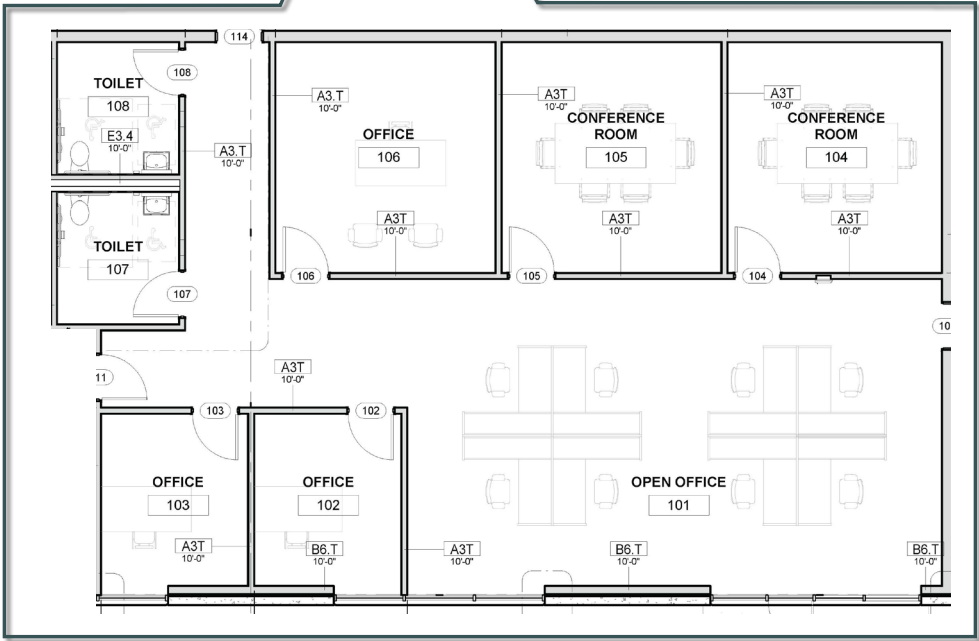
Office Floor Plan: 2,072 SF
