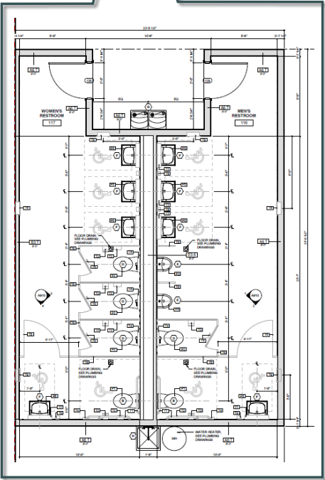
Office Floor Plan: Build to Suit 4 Men's and 4 Women's Restrooms Existing
