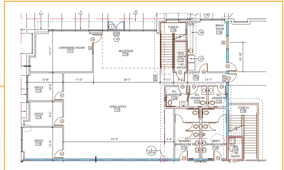
1st Floor Floorplan
