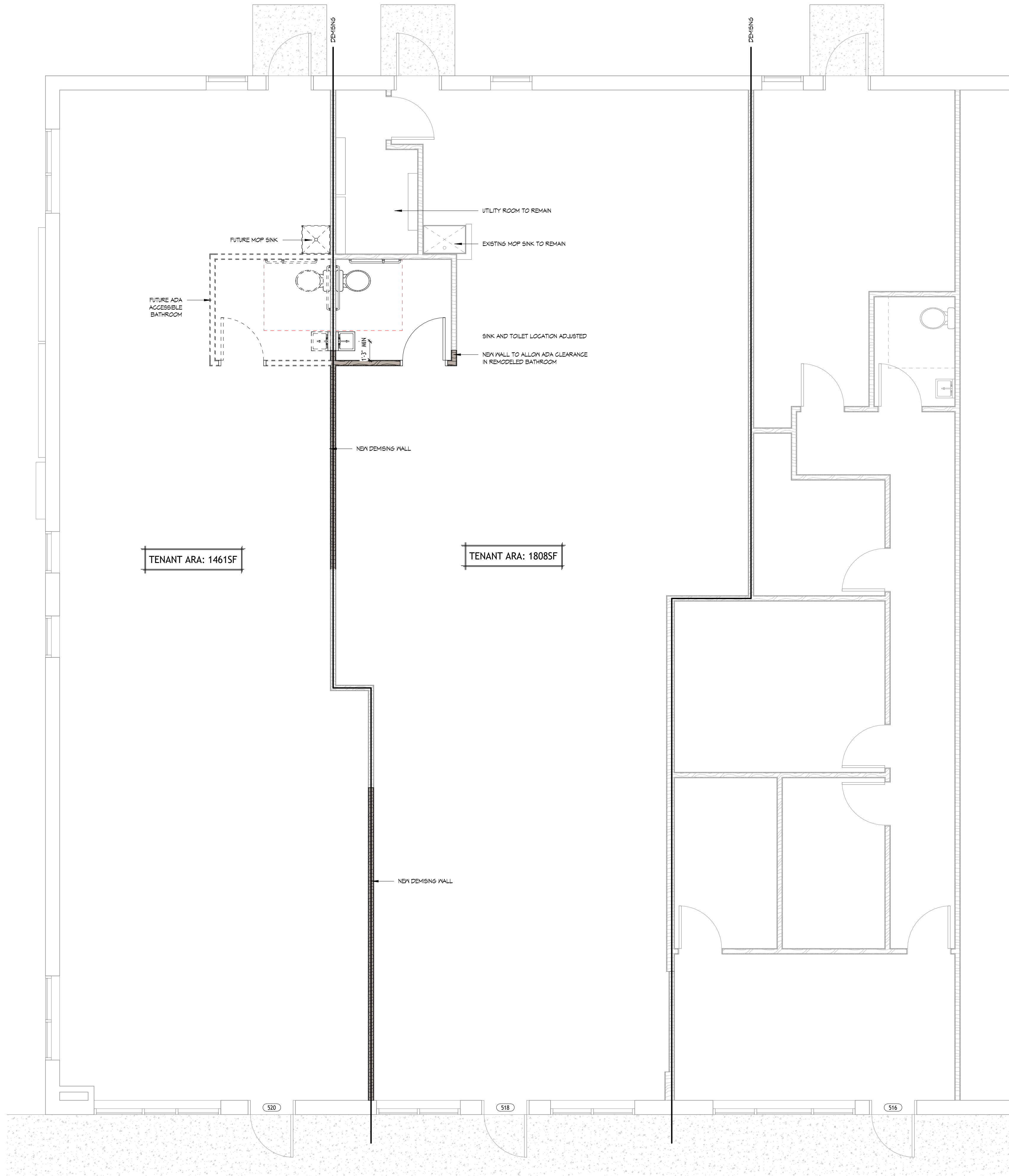
1 FLOOR PLAN - OPTION A A-1.1 1/4" = 1'-0"
