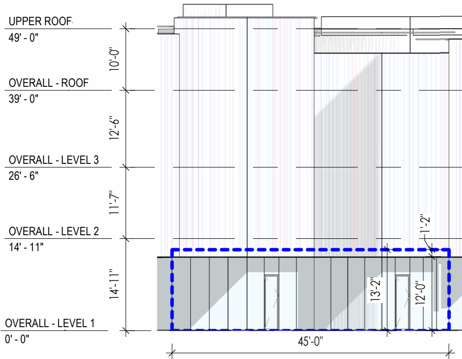
3 SOUTH ELEVATION - RETAIL R04 SCALE: 1/16" = 1'-0"
